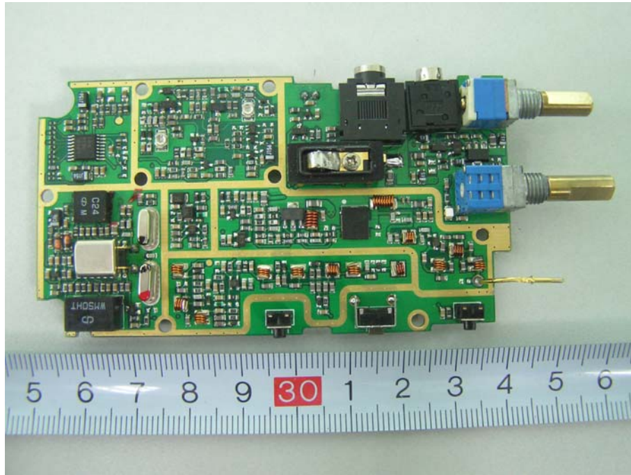
EUT –PCB Back View
