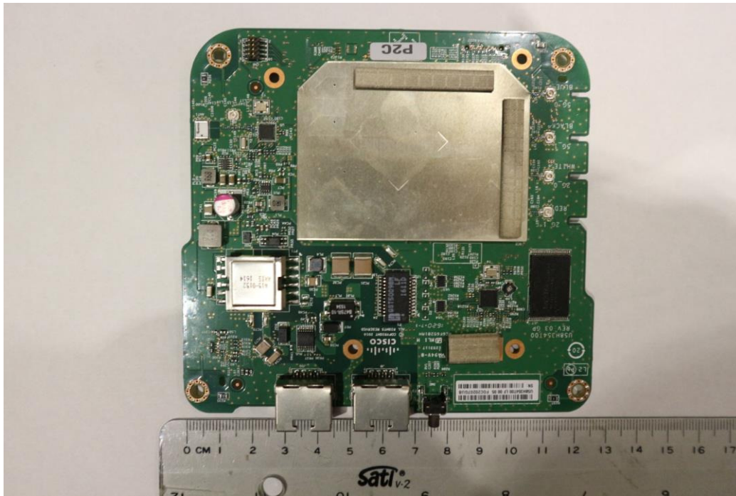
Top Side RF Board with shields
