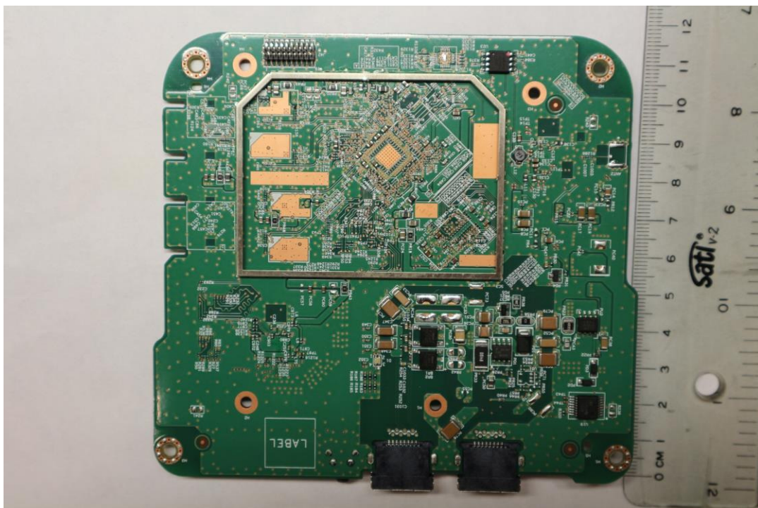
Bottom Side RF Board without Shields
