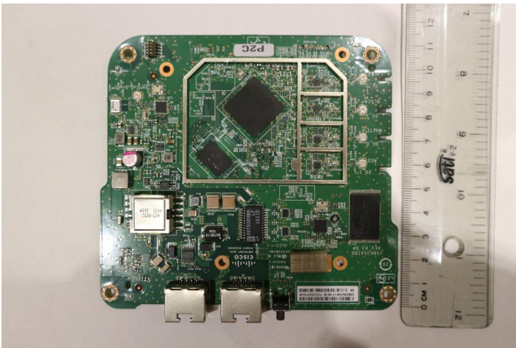
Top Side RF Board without Shields
