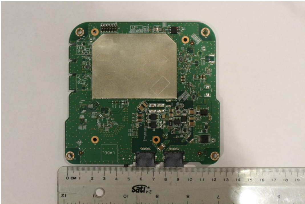
Bottom Side RF Board with Shields
