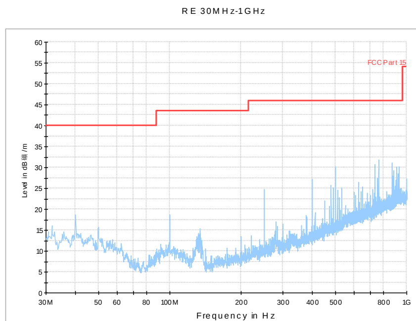
Fig. 259 Radiated Spurious Emission (802.11n-HT20, Ch11, 30 MHz-1 GHz)
