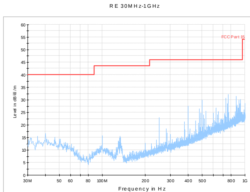
Fig. 271 Radiated Spurious Emission (802.11n-HT40, Ch3, 30 MHz-1 GHz)
