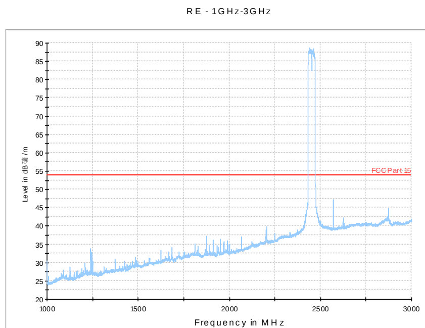
Fig. 279 Radiated Spurious Emission (802.11n-HT40, Ch9, 1 GHz-3 GHz)
