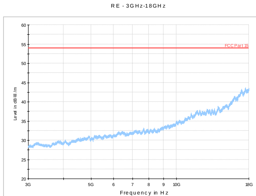
Fig. 257 Radiated Spurious Emission (802.11n-HT20, Ch6, 3 GHz-18 GHz)
