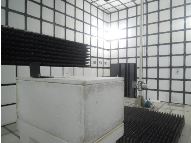
FCC_15_247_BT_Radiated_Setup_1
