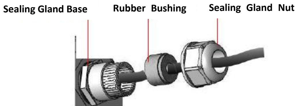
Inserting the Cable into the Sealing Cap
