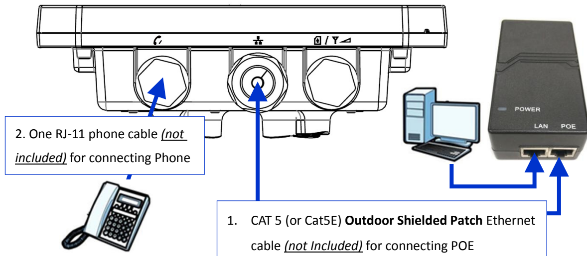
Figure 2: CPE Connections
