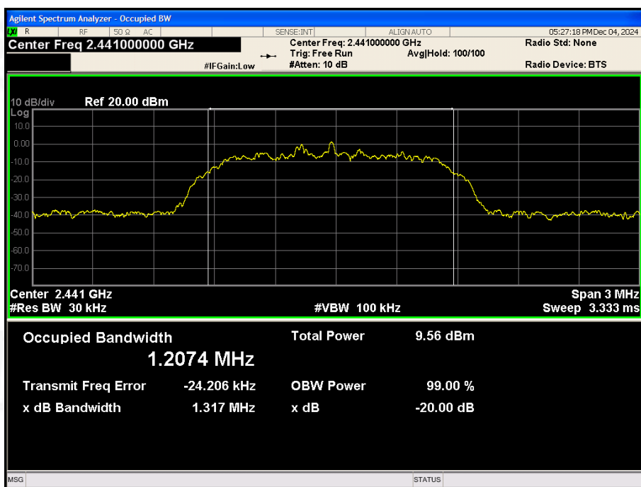
CH39: 2441MHz
