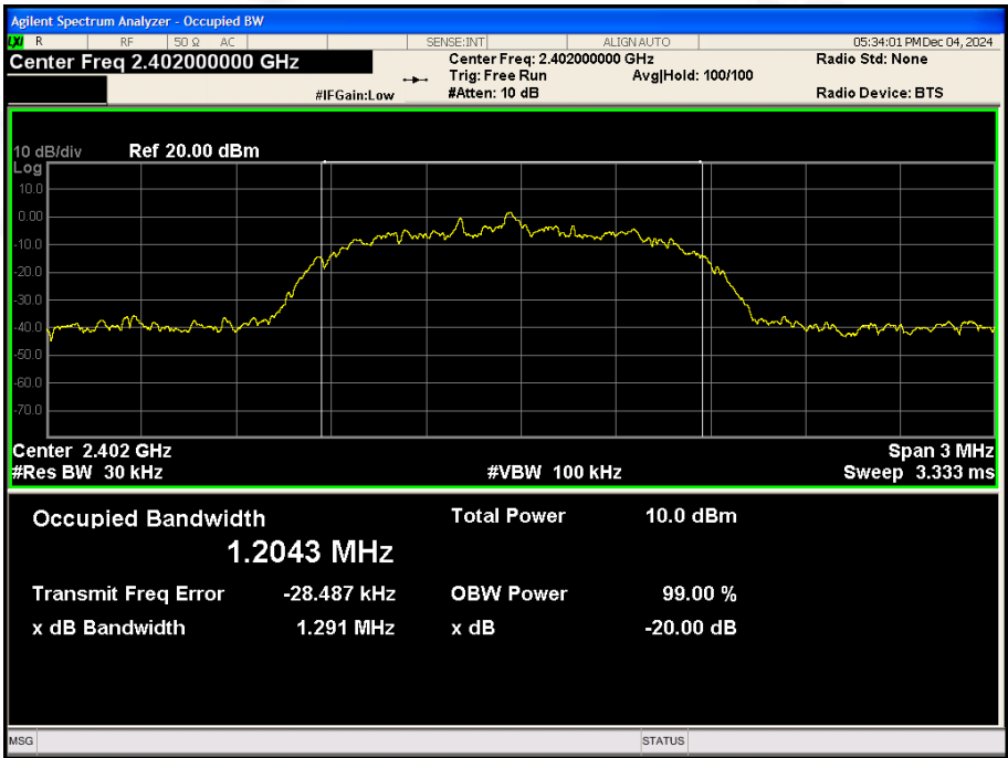
CH00: 2402MHz
