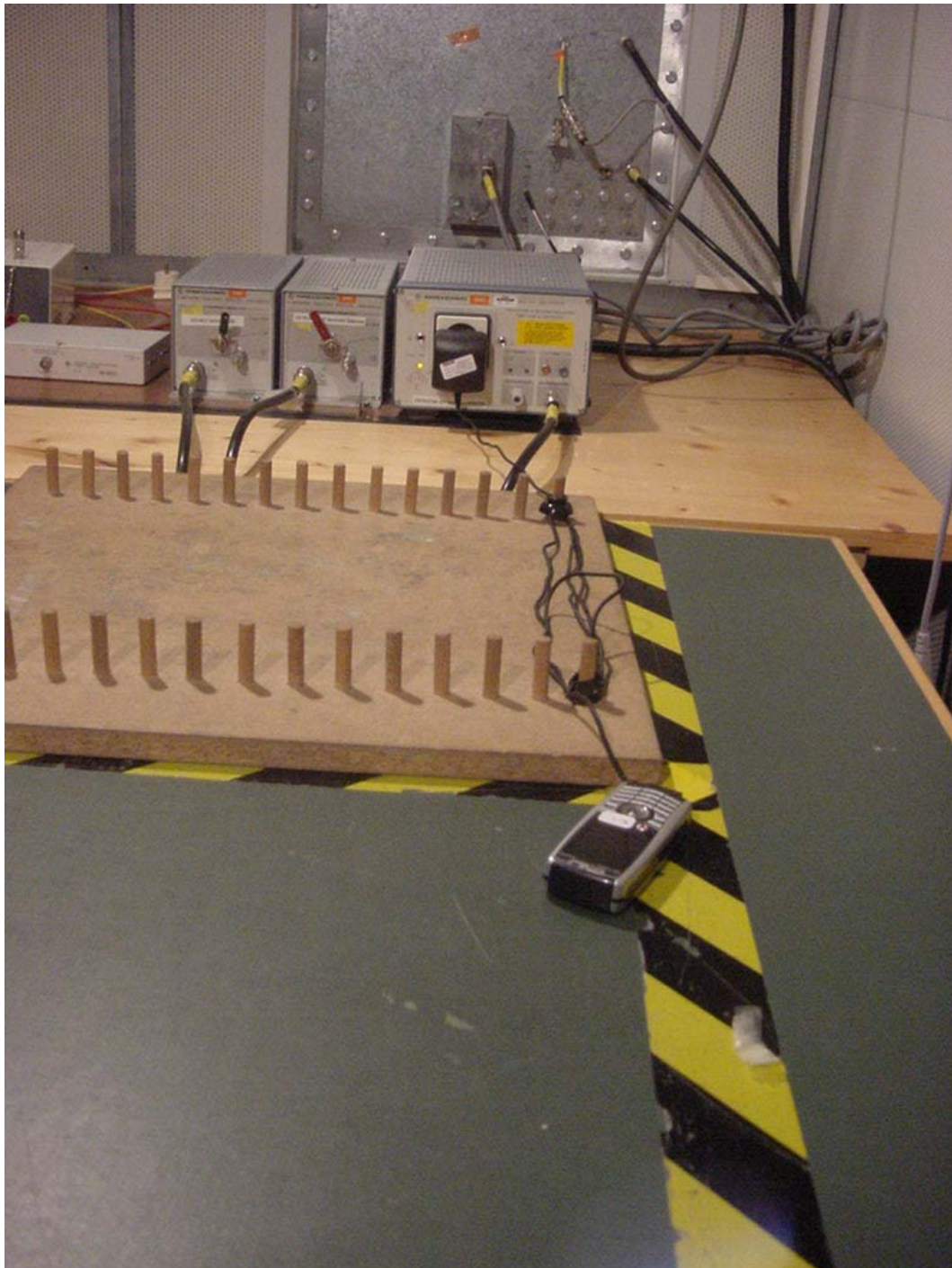
Photo 3: Conducted Emissions
