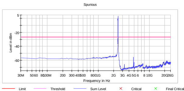
Conducted Emissions Ch06 802.11n HT40 MCS8 MIMO
