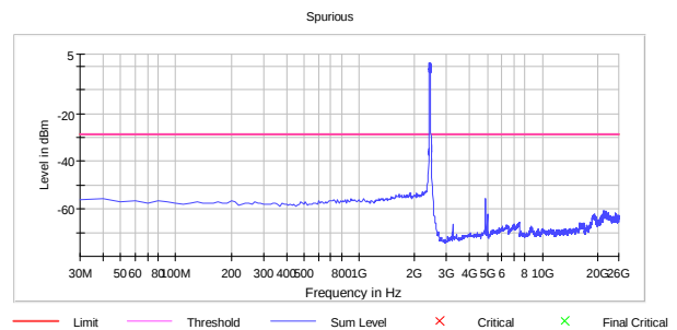
Conducted Emissions Ch06 802.11n HT40 MCS15 MIMO
