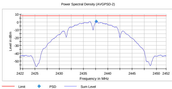
PSD, 2437 MHz, 802.11b 1M 0.64
