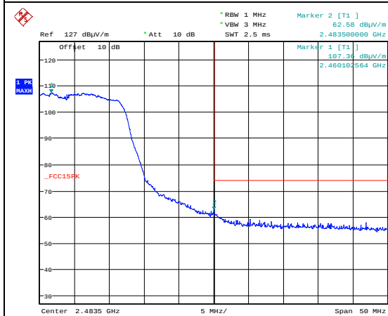
Band Edge, 2462 MHz, 802.11n MCS0, SISO, Peak
