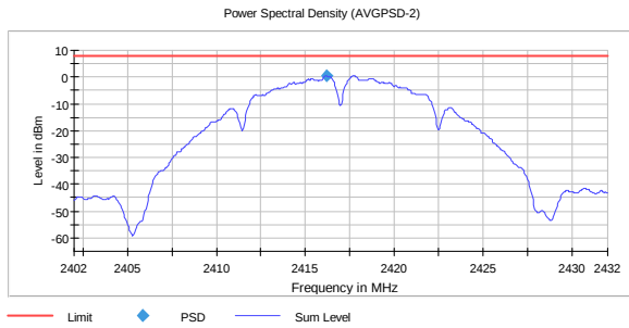
PSD, 2417 MHz, 802.11b 1M 0.45
