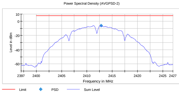
PSD, 2412 MHz, 802.11b 1M -6.20
