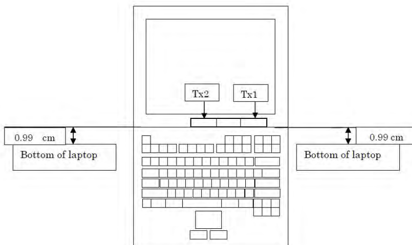
Fig.6 Antenna position of EUT (Front view)
