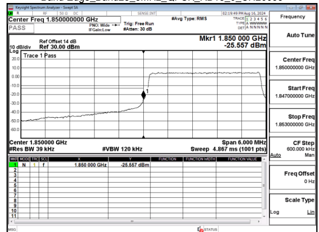
Band Edge_Band25_3MHz_QPSK_RB15_0_CH26055
