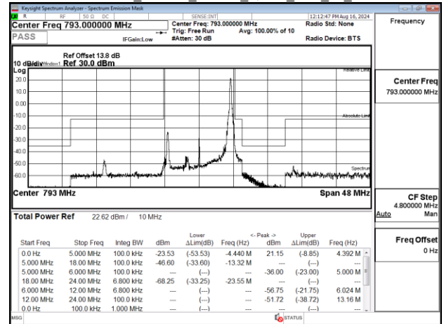
Emission Mask_Band14_10MHz_QPSK_RB50_0_CH23330
