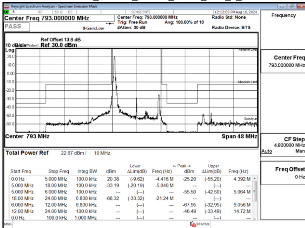
Emission Mask_Band14_10MHz_QPSK_RB1_0_CH23330
