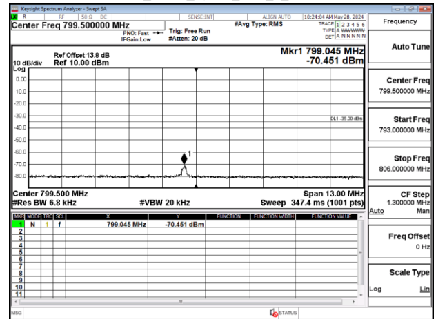
Band13_5MHz_QPSK_RB1_0_CH23255
