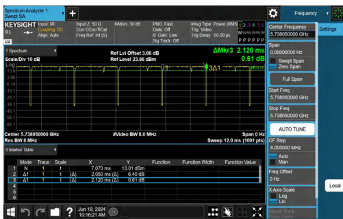
NTNV-11AX20SISO-Ant1-5745-26Tone-RU4
