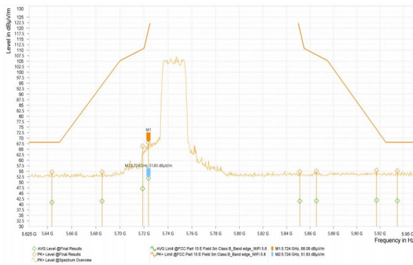
Wi-Fi 5G_11AX20_5745
