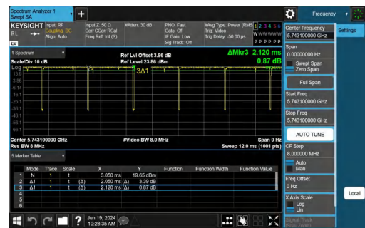
NTNV-11AX20SISO-Ant1-5745-52Tone-RU39
