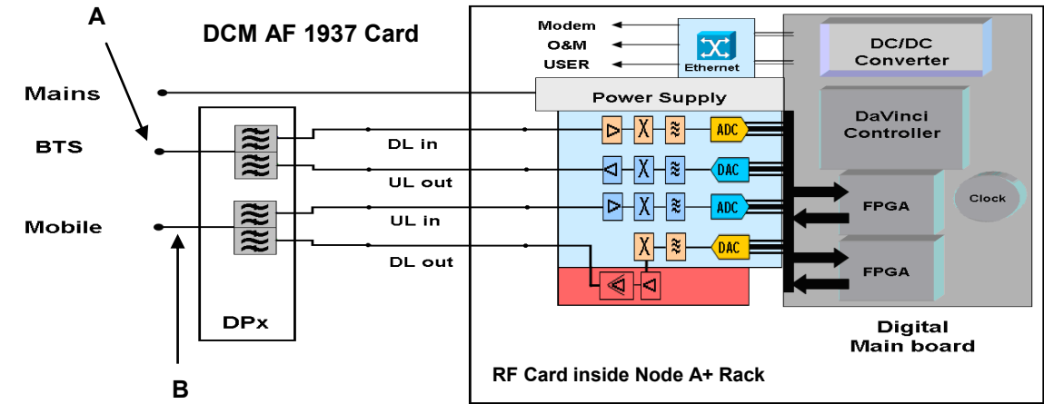
figure 2.1.4-#1 Block diagram of measurement reference points
