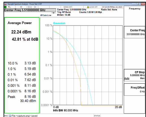
n77(3450-3550MHz) 80M DFT-s-OFDM 256QAM Outer_Full High
