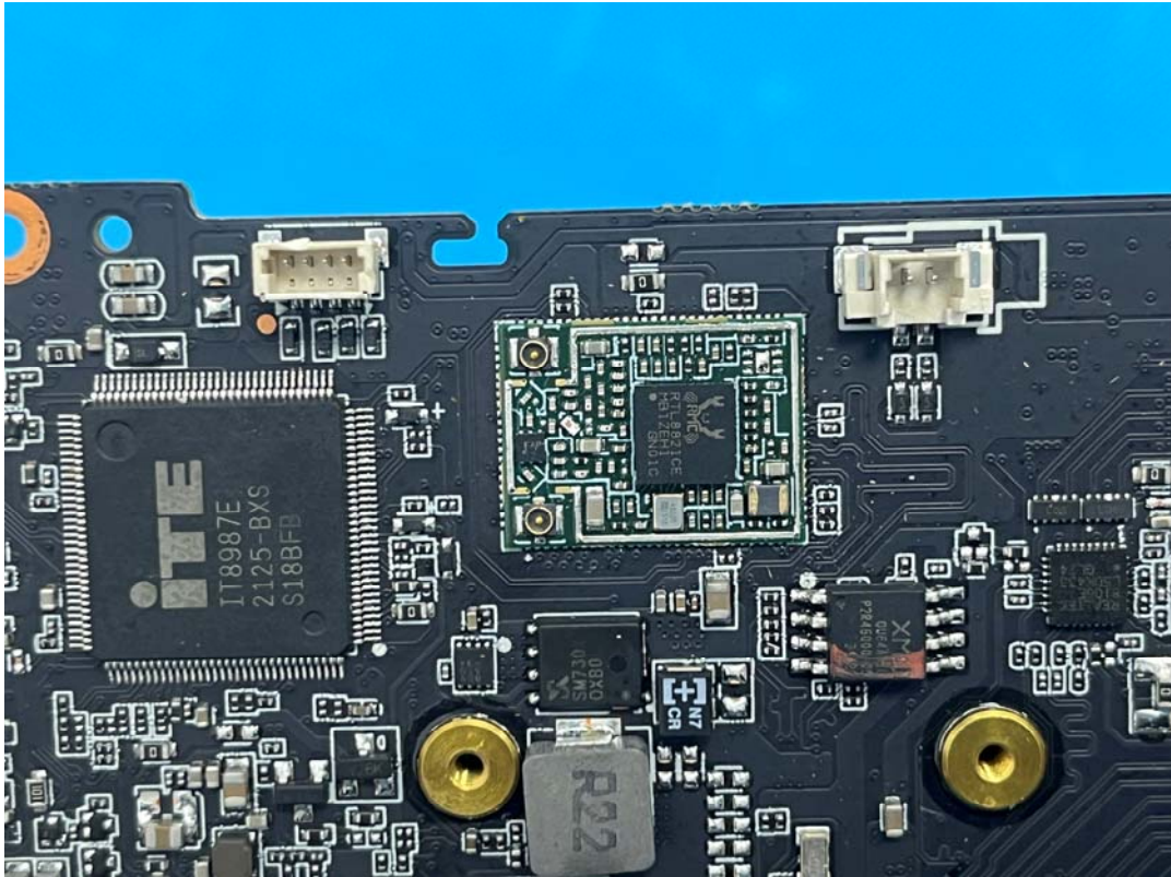
RF Module unshielded View
