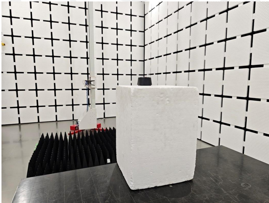
Spurious Radiation Emissions Test (>1G)
