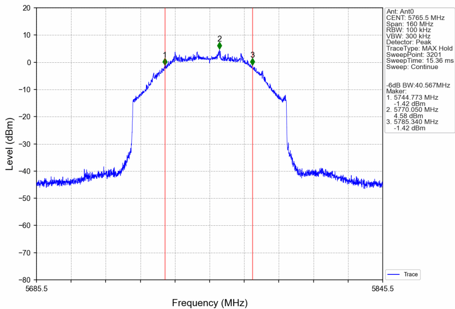
80M_LCH_5765.5MHz_Ant0_NTNV
