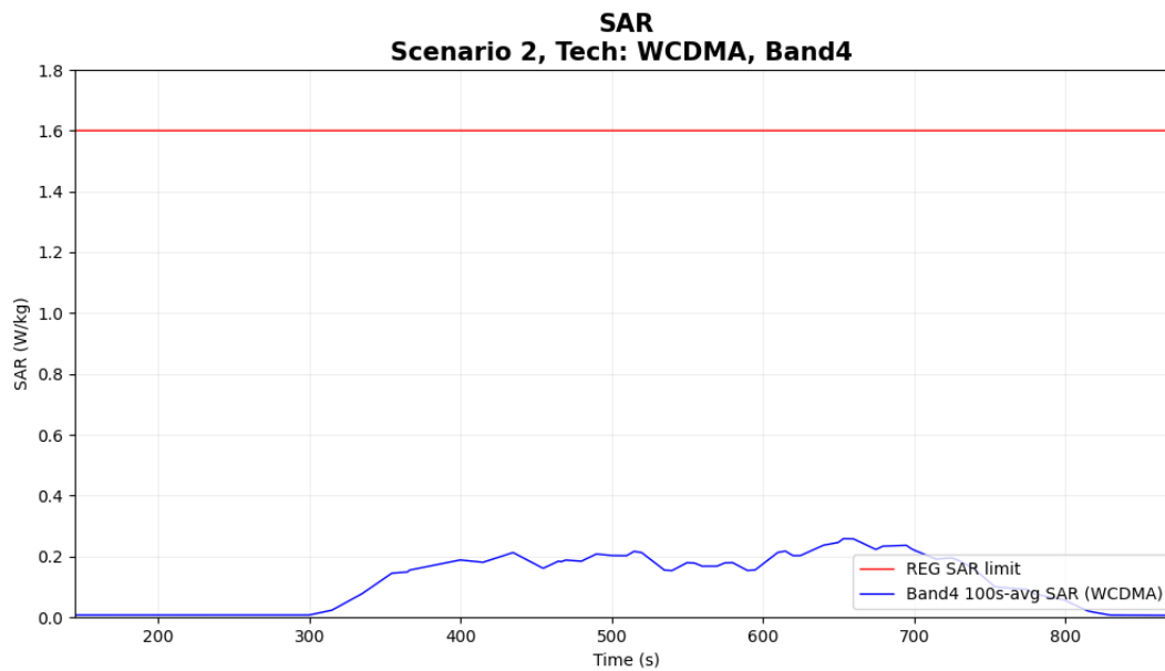
Figure 6-14 Time-averaged SAR
