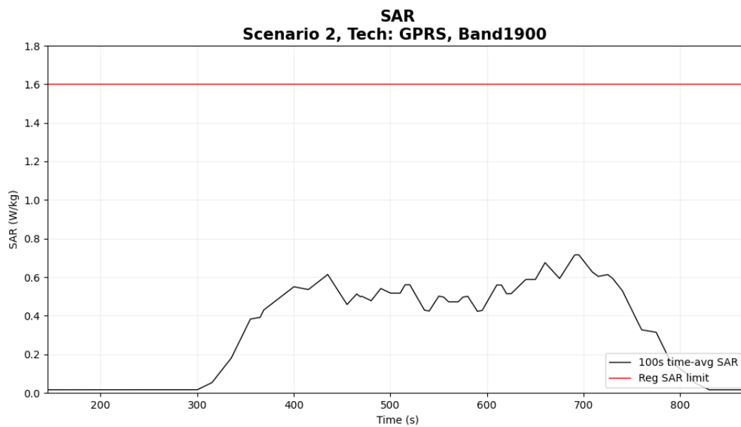
Figure 5- 14 Time-averaged SAR
