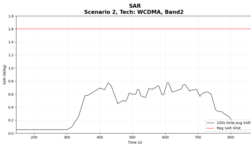
Figure 5- 17 Time-averaged SAR
