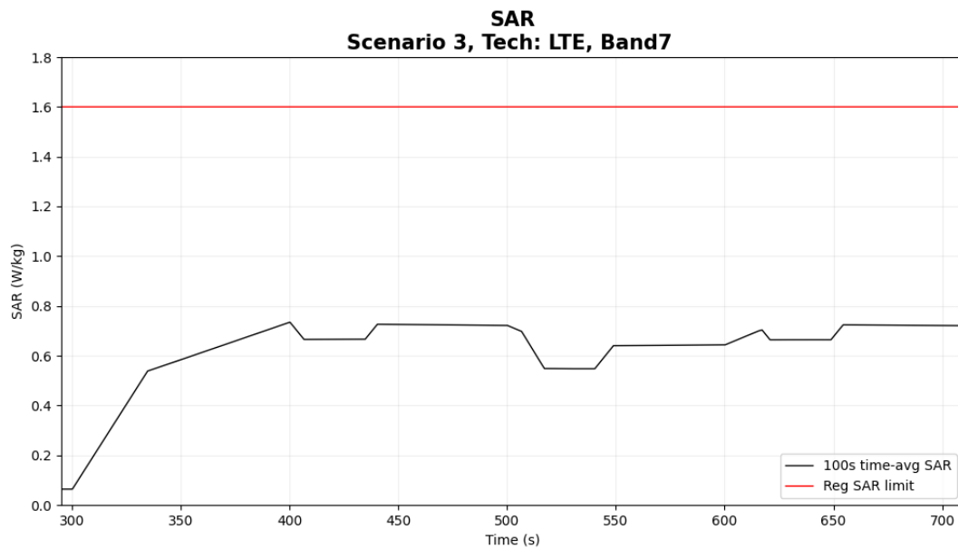
Figure 5- 37 Time-averaged SAR
