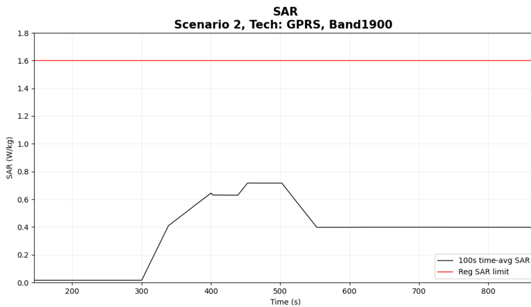
Figure 5- 12 Time-averaged SAR
