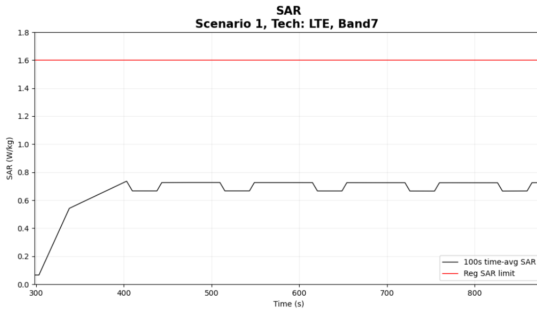
Figure 5- 6 Time-averaged SAR
