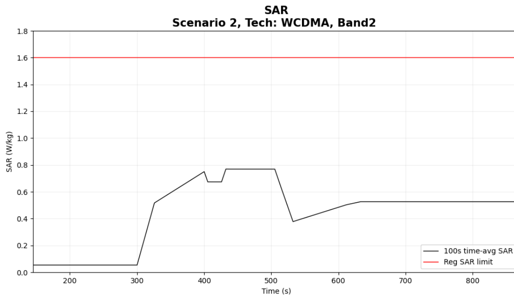
Figure 6- 16 Time-averaged SAR
