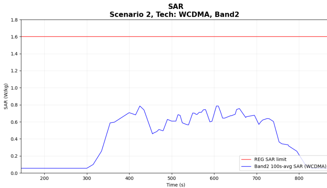
Figure 6-12 Time-averaged SAR
