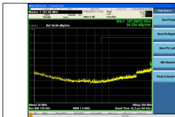
30-200 MHz Vertical
