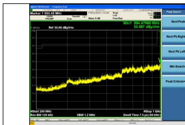
200-1000 MHz Vertical
