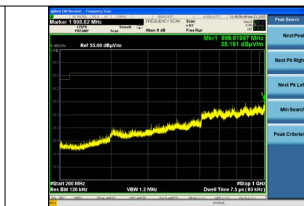
200-1000 MHz Horizontal
