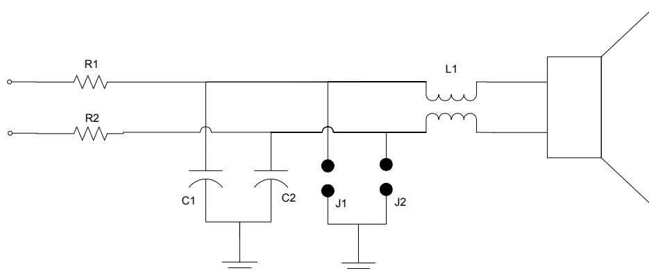
Figure 6 Earphone application circuit
