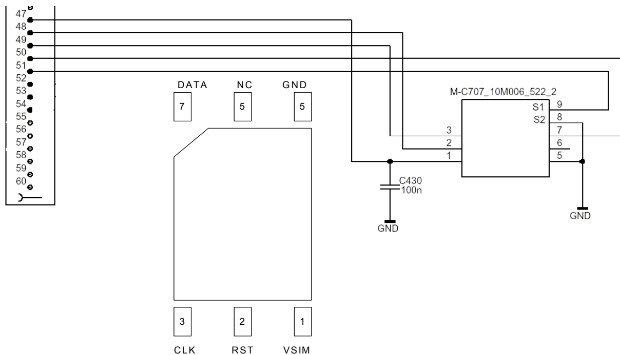
Figure 4 SIM connections
