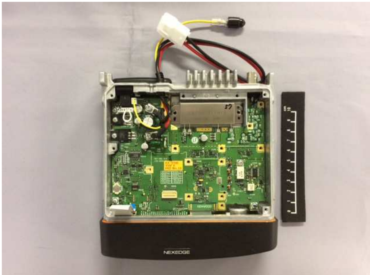
Top Internal View of Main Unit (without shield case)
