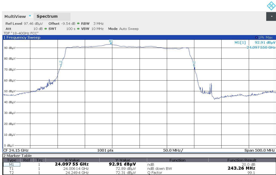
Plots No. 13: 20dB Bandwidth, Horizontal / Vertical Polarization
