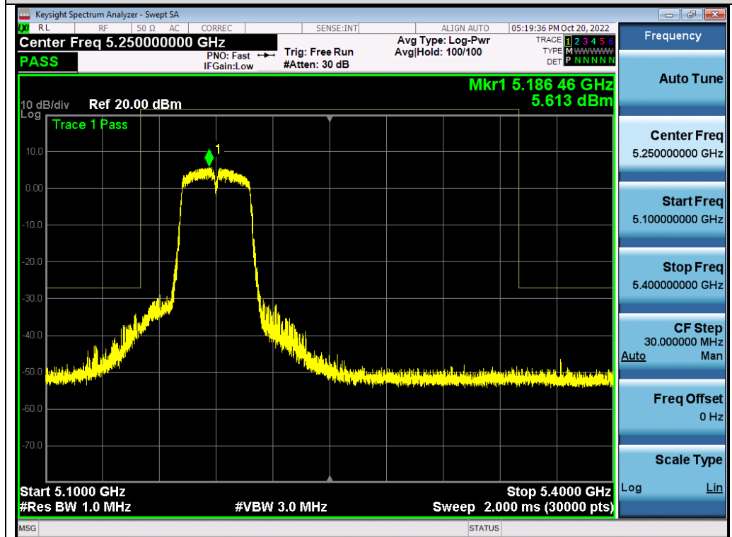
Test_Graph_802.11n40_ANT2_5190_MCS0_Frequency Band 3
