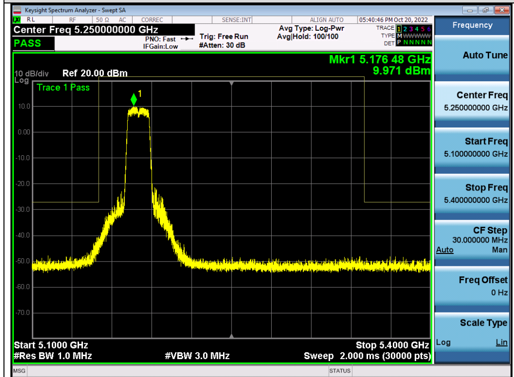
Test_Graph_802.11a_ANT2_5180_6Mbps_Frequency Band 3
