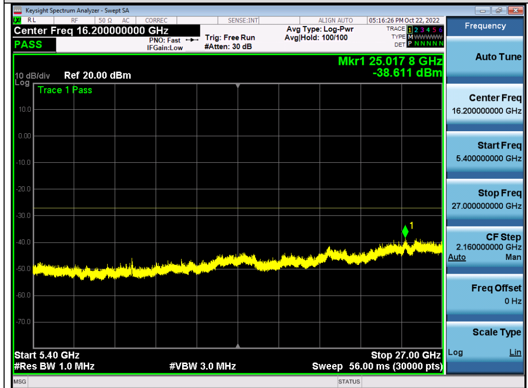
Test_Graph_802.11n40_ANT2_5310_MCS0_Frequency Band 4
