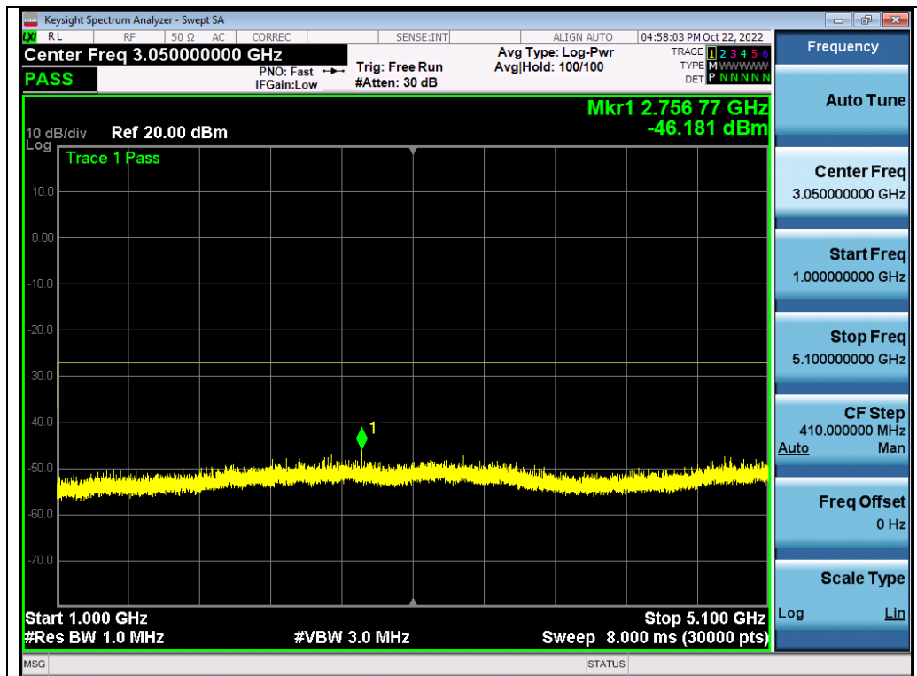
Test_Graph_802.11a_ANT2_5260_6Mbps_Frequency Band 2
