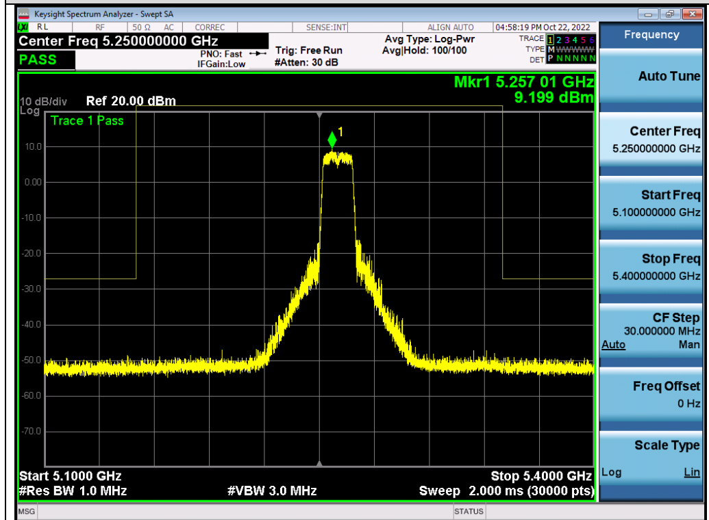
Test_Graph_802.11a_ANT2_5260_6Mbps_Frequency Band 3
