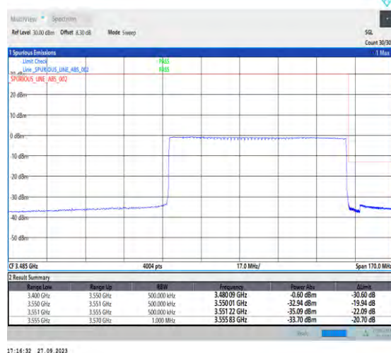
1-N78-3450-3550-PC2-30-80-H-6-CP-QPSK-Outer_Full-217@0-Ant7-1--PASS-see graph
