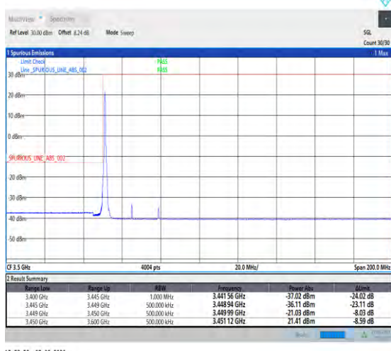
1-N78-3450-3550-PC2-30-30-L-4-CP-QPSK-Edge_1RB_Left-1@0-Ant7-1--PASS-see graph
