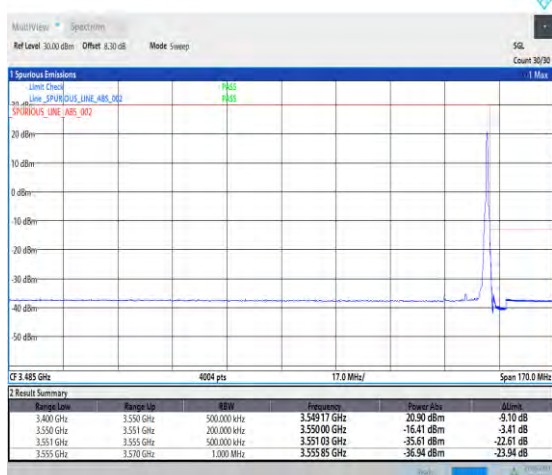
1-N78-3450-3550-PC2-30-15-H-5-CP-QPSK-Edge_1RB_Right-1@37-Ant7-1--PASS-see graph
