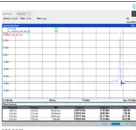
1-N78-3450-3550-PC2-30-10-H-2-DFT-PI2BPSK-Edge_1RB_Right-1@23-Ant7-1--PASS-see graph
