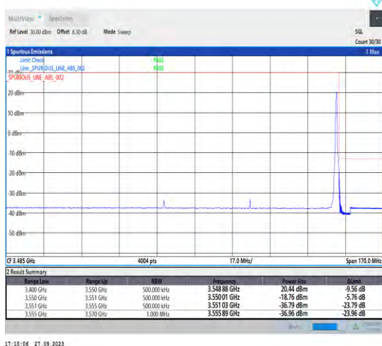
1-N78-3450-3550-PC2-30-80-H-5-CP-QPSK-Edge_1RB_Right-1@216-Ant7-1--PASS-see graph
