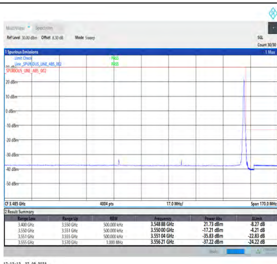
1-N78-3450-3550-PC2-30-80-H-2-DFT-PI2BPSK-Edge_1RB_Right-1@216-Ant7-1--PASS-see graph
