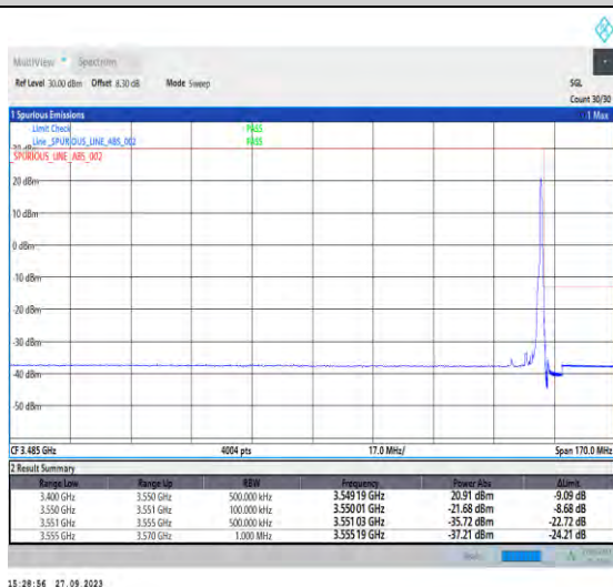
1-N78-3450-3550-PC2-30-10-H-5-CP-QPSK-Edge_1RB_Right-1@23-Ant7-1--PASS-see graph
