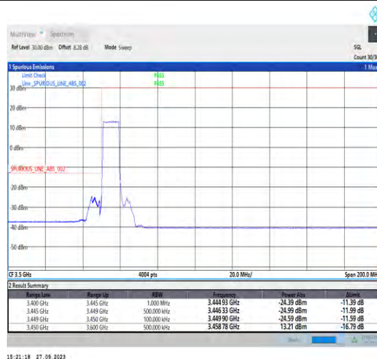
1-N78-3450-3550-PC2-30-10-L-3-DFT-PI2BPSK-Outer_Full-24@0-Ant7-1--PASS-see graph
