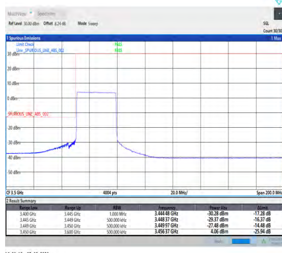
1-N78-3450-3550-PC2-30-30-L-6-CP-QPSK-Outer_Full-78@0-Ant7-1--PASS-see graph
