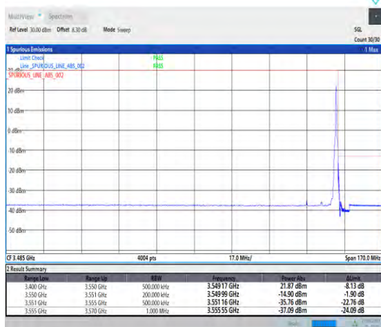
1-N78-3450-3550-PC2-30-15-H-2-DFT-PI2BPSK-Edge_1RB_Right-1@37-Ant7-1--PASS-see graph
