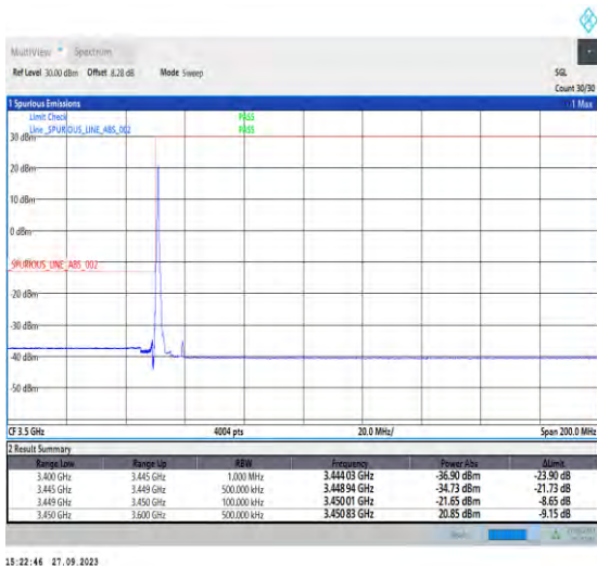
1-N78-3450-3550-PC2-30-10-L-4-CP-QPSK-Edge_1RB_Left-1@0-Ant7-1--PASS-see graph
