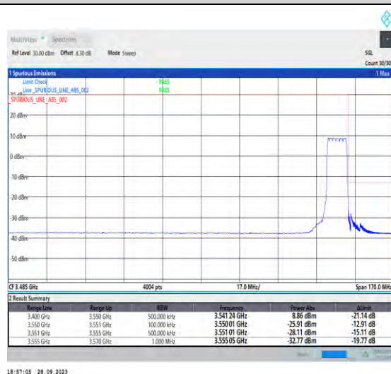
1-N78-3450-3550-PC2-30-10-H-6-CP-QPSK-Outer_Full-24@0-Ant7-1--PASS-see graph
