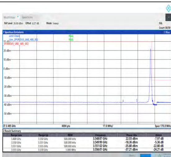
1-N78-3450-3550-PC2-30-30-H-2-DFT-PI2BPSK-Edge_1RB_Right-1@77-Ant7-1--PASS-see graph
