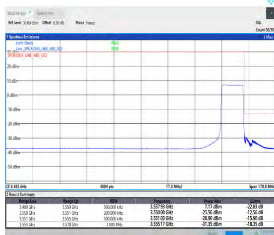
1-N78-3450-3550-PC2-30-15-H-6-CP-QPSK-Outer_Full-38@0-Ant7-1--PASS-see graph
