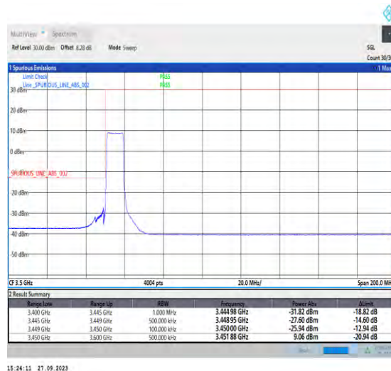
1-N78-3450-3550-PC2-30-10-L-6-CP-QPSK-Outer_Full-24@0-Ant7-1--PASS-see graph
