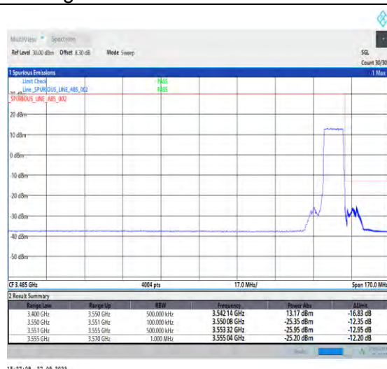
1-N78-3450-3550-PC2-30-10-H-3-DFT-PI2BPSK-Outer_Full-24@0-Ant7-1--PASS-see graph
