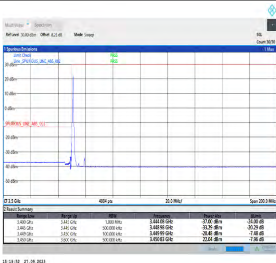
1-N78-3450-3550-PC2-30-10-L-1-DFT-PI2BPSK-Edge_1RB_Left-1@0-Ant7-1--PASS-see graph
