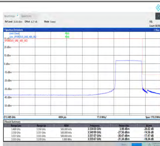
1-N78-3450-3550-PC2-30-30-H-3-DFT-PI2BPSK-Outer_Full-75@0-Ant7-1--PASS-see graph
