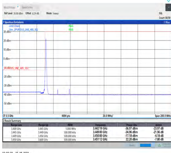
1-N78-3450-3550-PC2-30-30-L-1-DFT-PI2BPSK-Edge_1RB_Left-1@0-Ant7-1--PASS-see graph
