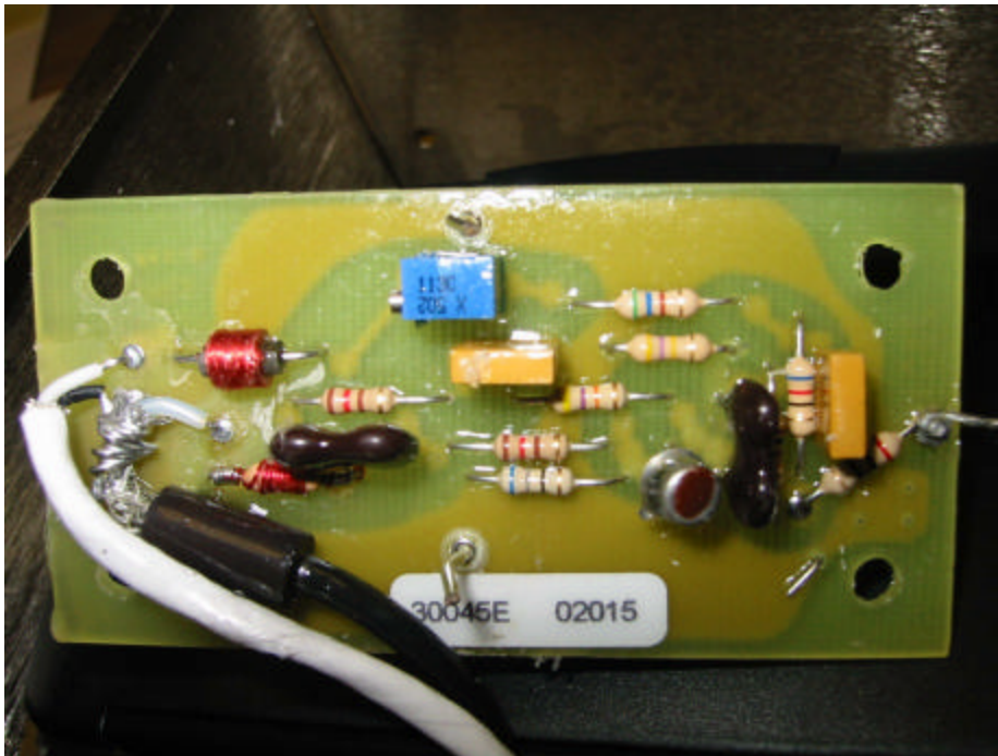
COMPONENT SIDE
