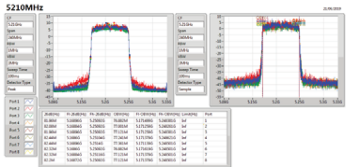
802.11ax HEW80_Nss1,(MCS0)_8TX
