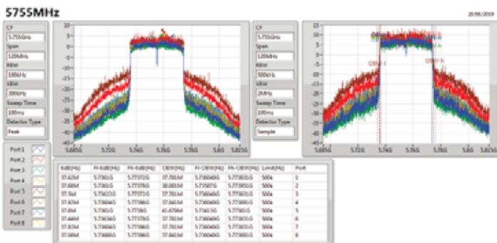
802.11ax HEW40_Nss1,(MCS0)_8TX
