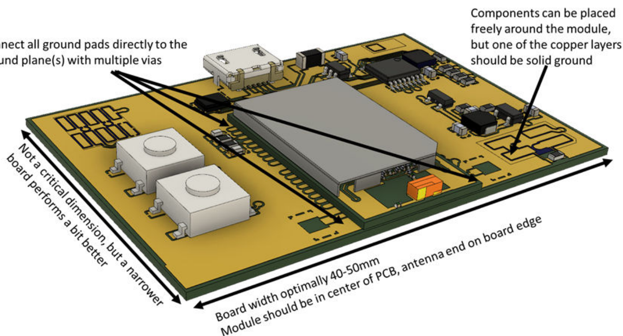
Figure 5.4. Details about Board Dimensions and Module Placement
