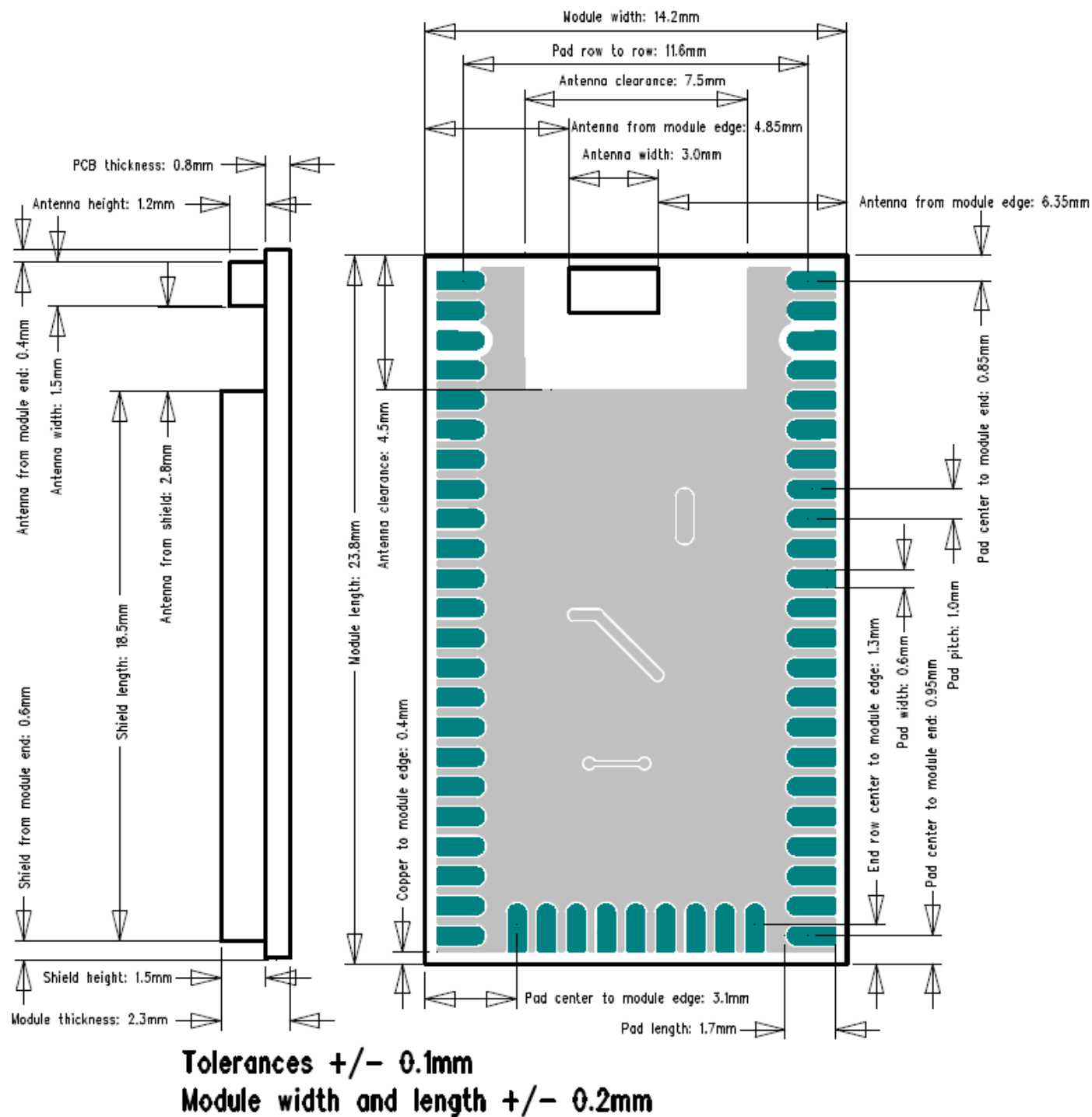
Figure 7.1. WGM160PX22KGA2 Package Outline
