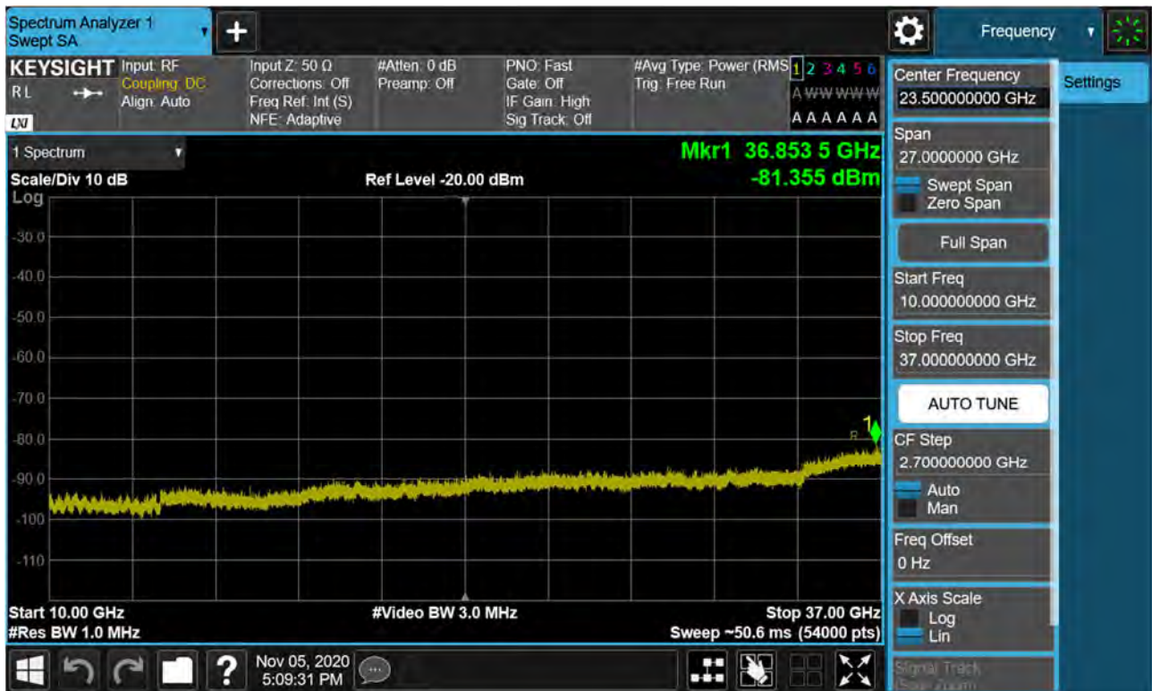
BAND 48. Conducted Spurious Plot 2 (5 MHz Ch. 56715 QPSK RB 1, Offset 0)
