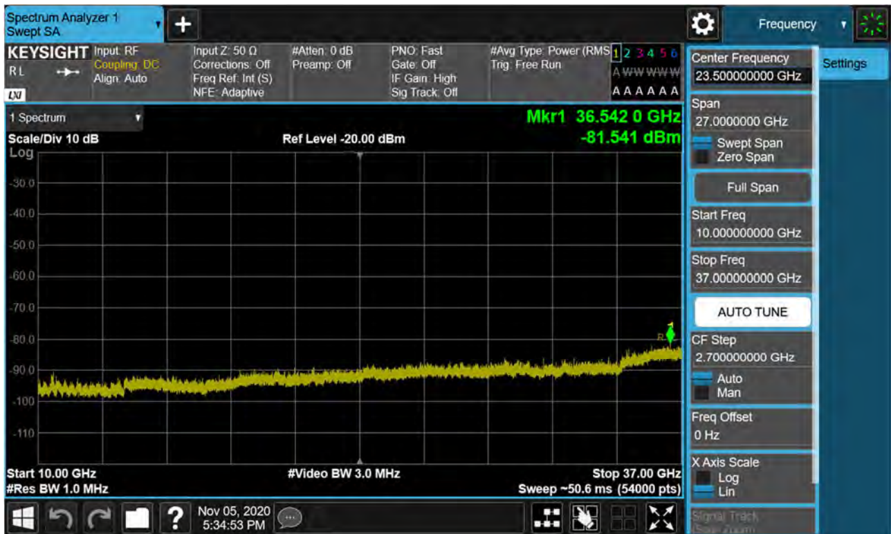
BAND 48. Conducted Spurious Plot 2 (15 MHz Ch. 55315 QPSK RB 1, Offset 0)
