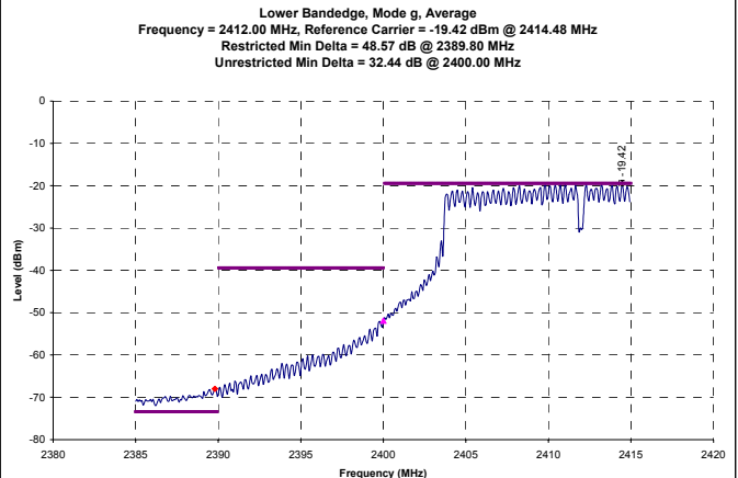
Channel 1 Mode g - Conducted Average Band-edge Plots
