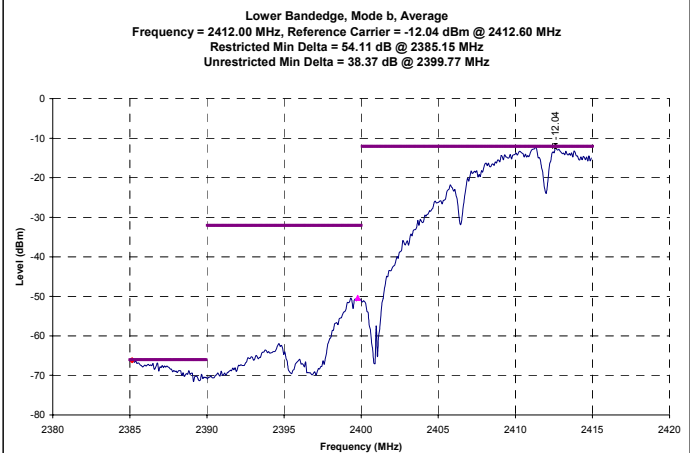
Channel 1 Mode b - Conducted Average Band-edge Plots
