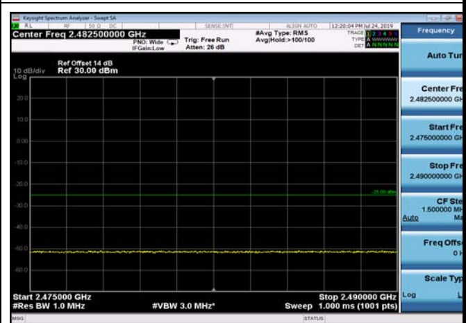
FDD07_10MHz_2565_QPSK_fullRB_ExtraBands_Range_2475~2490
