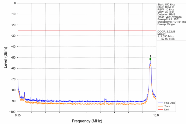
Band38 15MHz 16QAM LCH 2577.5MHz RB 1 0 NTN
