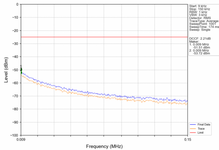
Band38_15MHz_QPSK_LCH_2577.5MHz_RB_1_0_NTV
