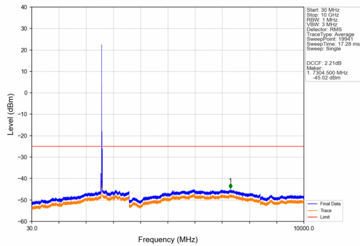
Band38_15MHz_QPSK_MCH_2595MHz_RB_1_0_NTNV
