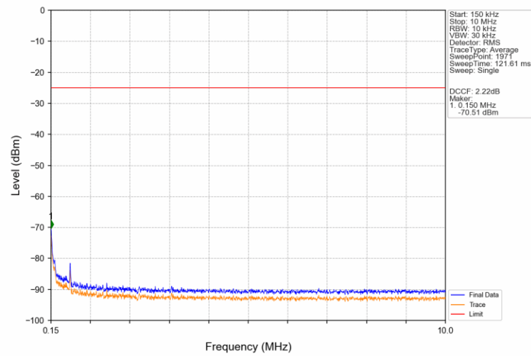
Band38_15MHz_16QAM_HCH_2612.5MHz_RB_1_0_NTNV
