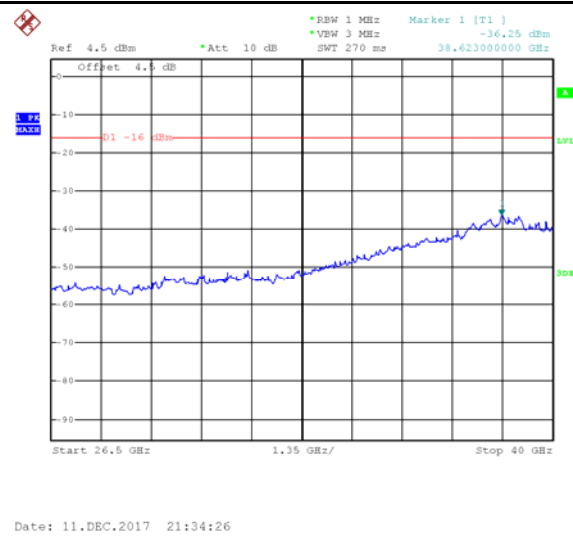
5MHz - High CH 26.5GHz~40GHz
