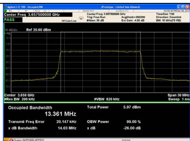
15MHz - Low CH 16QAM
