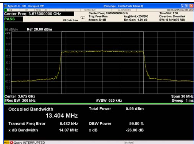
15MHz - Middle CH 16QAM
