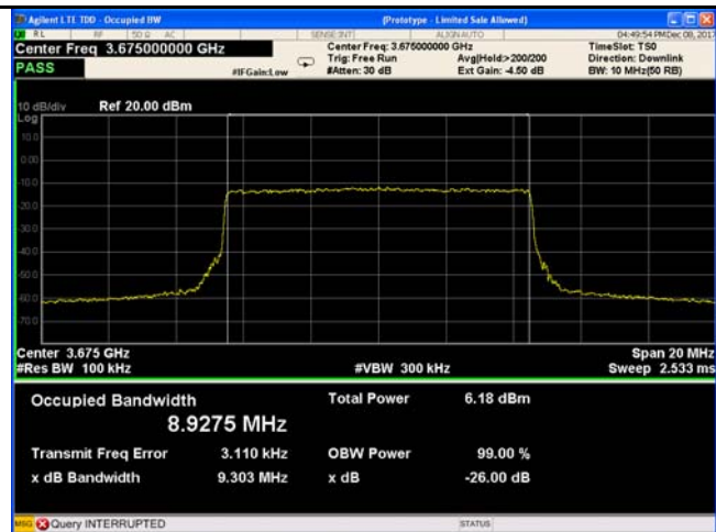
10MHz - Middle CH 16QAM
