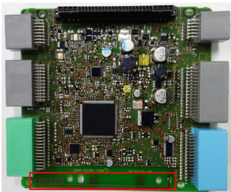
Figure 8.1 K72R0 PCB assy (top view) ※Pattern antenna is in red frame
