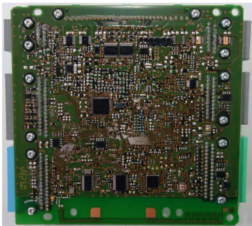
Figure 8.2 K72R0 PCB assy (bottom view)
