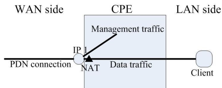
NAT mode, choosing “ Combine ” in WAN MGMT and Data Interface
