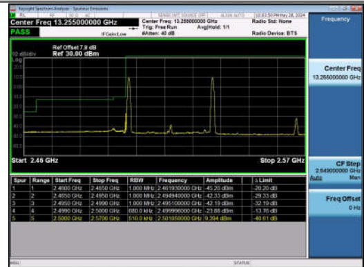
20MHz-15MHz_QPSK@QPSK-QPSK@QPSK_20850-210 21_1RB#0@100RB#0-1RB#74@75RB#0
