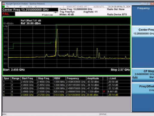
20MHz-20MHz_QPSK@QPSK-QPSK@QPSK_20850-21 048_1RB#0@100RB#0-0RB#0@100RB#0
