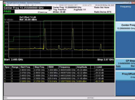
20MHz-10MHz_QPSK@QPSK-QPSK@QPSK_20850-20994_1RB#0@100RB#0-1RB#49@50RB#0
