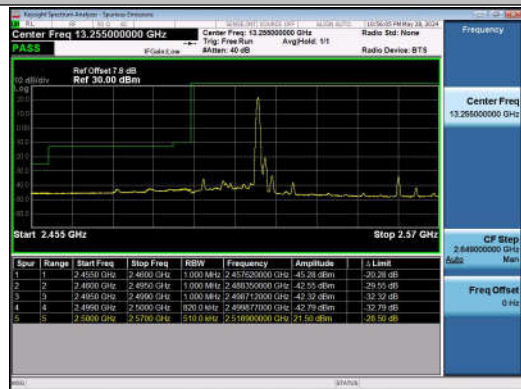
20MHz-20MHz_QPSK@QPSK-QPSK@QPSK_20850-210_48_1RB#99@100RB#0-0RB#0@100RB#0
