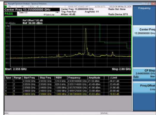
15MHz-15MHz_QPSK@QPSK-QPSK@QPSK_41015-41165 _1RB#74@75RB#0-0RB#0@75RB#0
