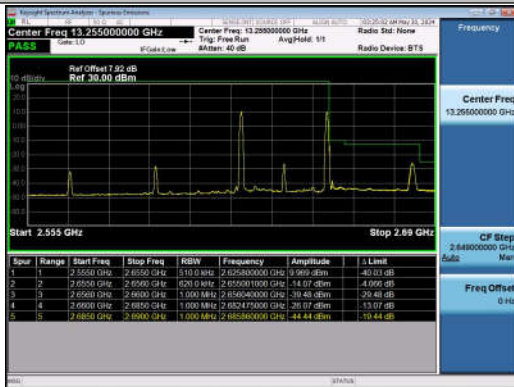
15MHz-15MHz_QPSK@QPSK-QPSK@QPSK_41015-41 165_1RB#0@75RB#0-1RB#74@75RB#0
