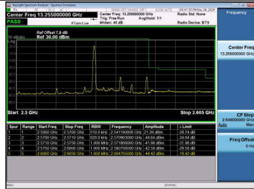
20MHz-10MHz_QPSK@QPSK-QPSK@QPSK_21251-21395_1RB#0@100RB#0-0RB#0@50RB#0
