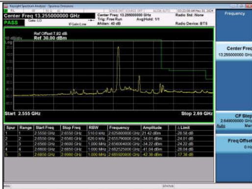
15MHz-15MHz_QPSK@QPSK-QPSK@QPSK_41015-41 165_1RB#0@75RB#0-0RB#0@75RB#0
