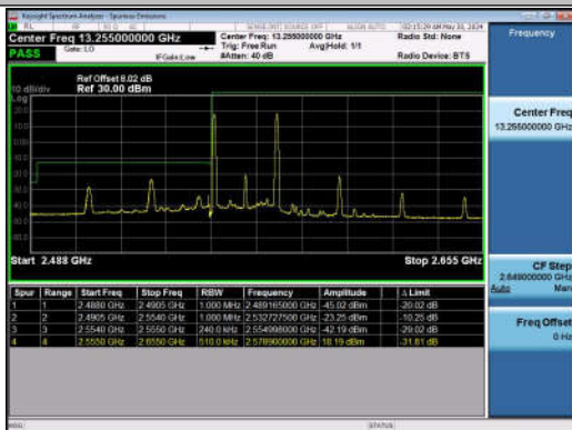
15MHz-10MHz_QPSK@QPSK-QPSK@QPSK_40315-40435_1RB#0@75RB#0-1RB#49@50RB#0
