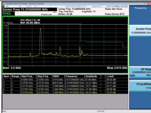
20MHz-20MHz_QPSK@QPSK-QPSK@QPSK_21152-21 350_1RB#0@100RB#0-0RB#0@100RB#0
