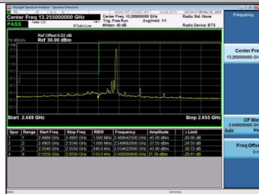
15MHz-10MHz_QPSK@QPSK-QPSK@QPSK_40315-40435_1RB#74@75RB#0-0RB#0@50RB#0
