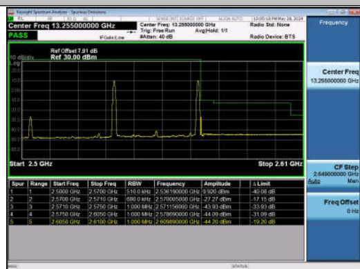
20MHz-15MHz_QPSK@QPSK-QPSK@QPSK_21201-213_72_1RB#0@100RB#0-1RB#74@75RB#0
