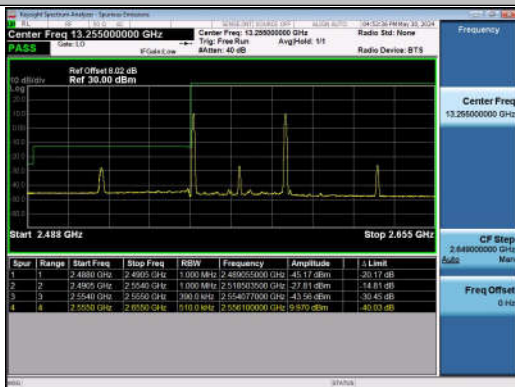
20MHz-20MHz_QPSK@QPSK-QPSK@QPSK_40340-40 538_1RB#0@100RB#0-1RB#99@100RB#0
