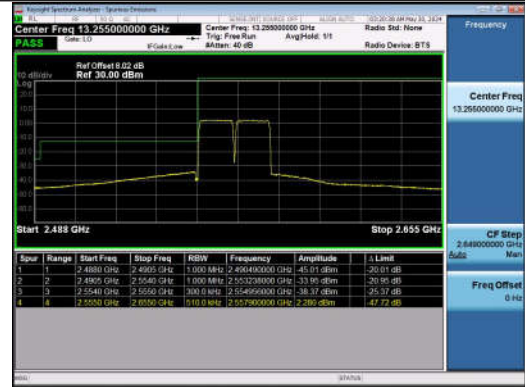
15MHz-15MHz_QPSK@QPSK-QPSK@QPSK_40315-40465 _75RB#0@75RB#0-75RB#0@75RB#0
