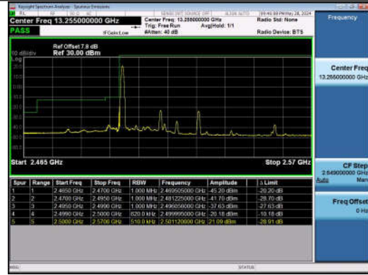
20MHz-10MHz_QPSK@QPSK-QPSK@QPSK_20850-20994_1RB#0@100RB#0-0RB#0@50RB#0
