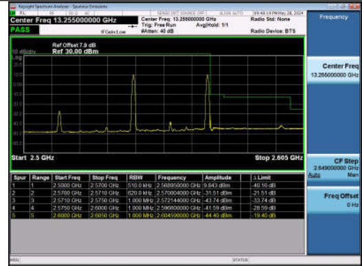
20MHz-10MHz_QPSK@QPSK-QPSK@QPSK_21251-213 95_1RB#0@100RB#0-1RB#49@50RB#0
