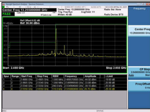
15MHz-10MHz_QPSK@QPSK-QPSK@QPSK_40315-40435_1RB#0@75RB#0-0RB#0@50RB#0
