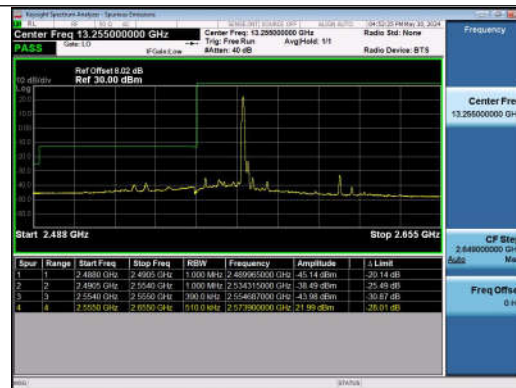
20MHz-20MHz_QPSK@QPSK-QPSK@QPSK_40340-40538 _1RB#99@100RB#0-0RB#0@100RB#0
