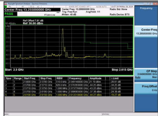
20MHz-20MHz_QPSK@QPSK-QPSK@QPSK_21152-21350 _1RB#99@100RB#0-0RB#0@100RB#0
