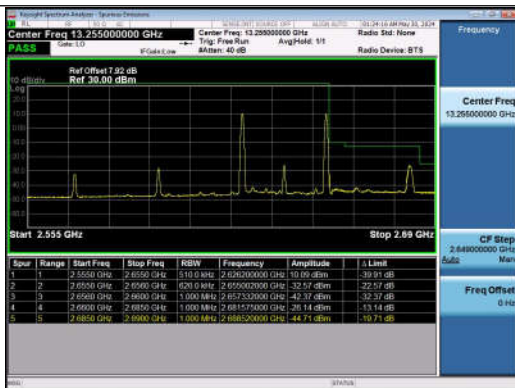
10MHz-20MHz_QPSK@QPSK-QPSK@QPSK_40996-41140_1RB#0@50RB#0-1RB#99@100RB#0
