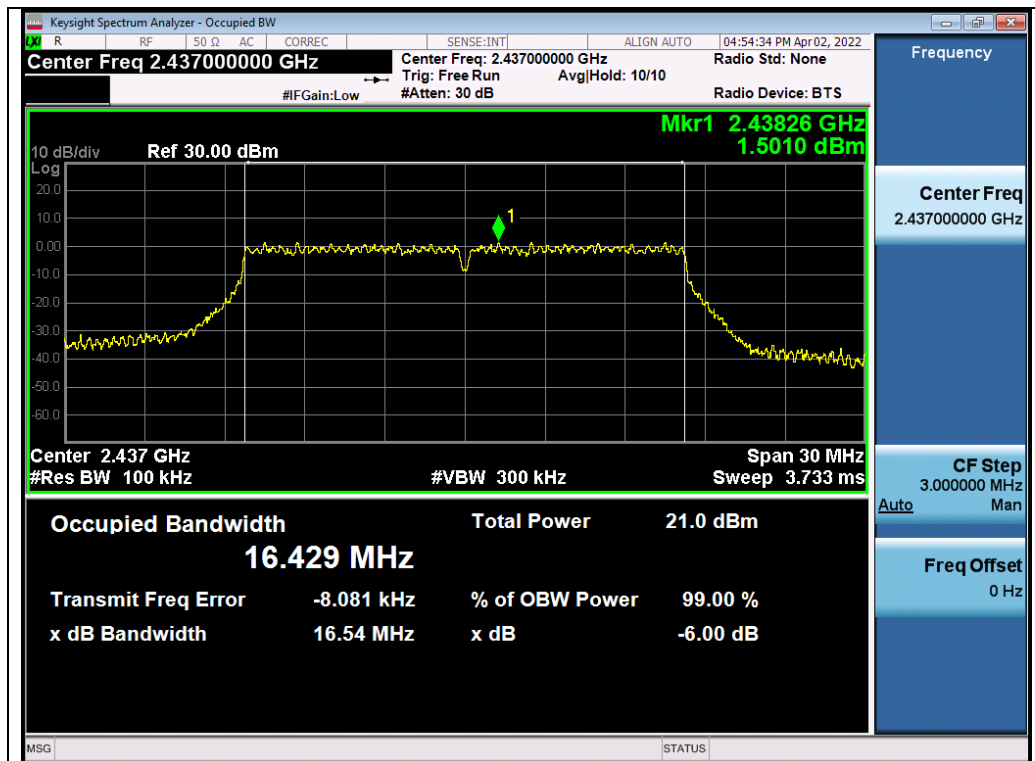
Test_Graph_802.11g_ANT1_2437_6Mbps_DTSCW
