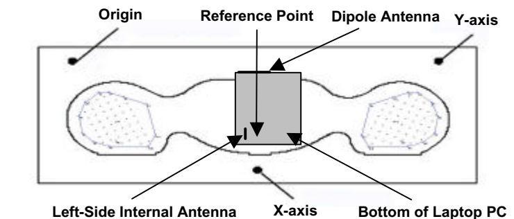
Figure 4. Phantom Reference Point & EUT Positioning Bottom Left Side of Laptop PC (LCD Display Closed)- Left-Side Antenna
