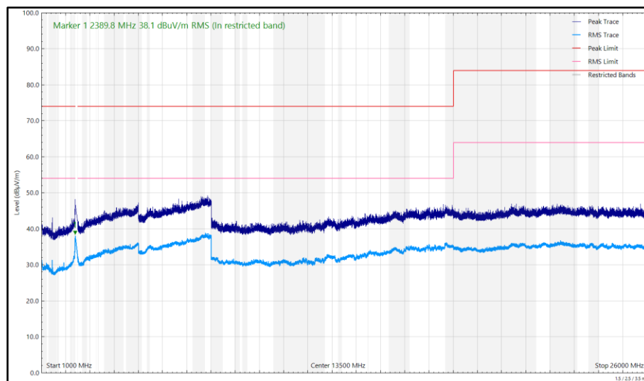
Figure 262 - 2402 MHz (CH37), LE1M, iPA, Core 0 + Core 1, 1 GHz to 26 GHz, Vertical
