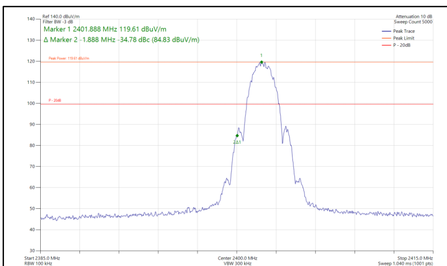
Figure 259 - Bluetooth LE2M, MIMO, Core 0 - Core 1 - 2402 MHz Band Edge Frequency 2400 MHz
