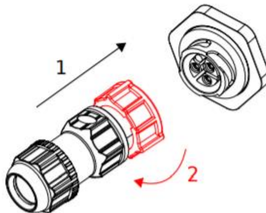
Figure 2.5: Power Connector
