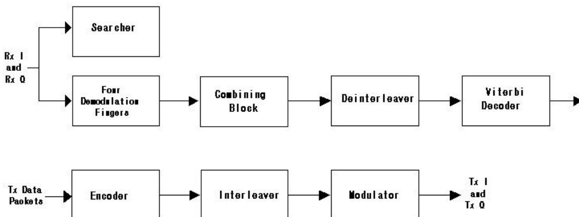
Figure 3-3. CDMA digital Baseband Block Diagram
