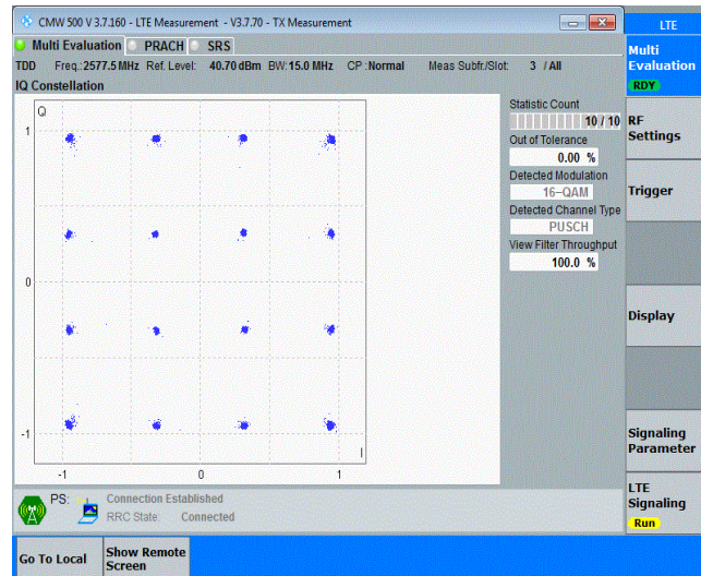
Band38-15MHz-16QAM-38000-75RB#0
