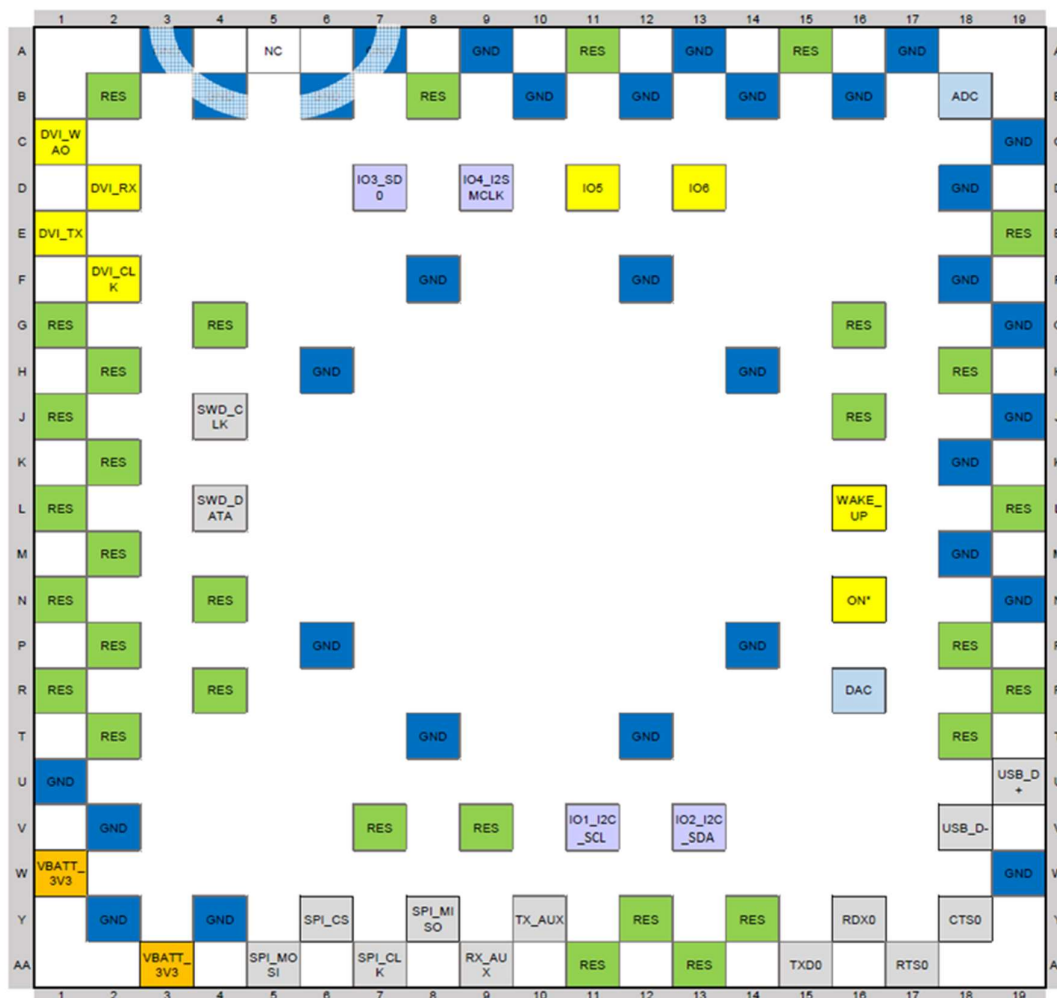
Figure 3: Telit WE310G4-I Pads Layout Top View
