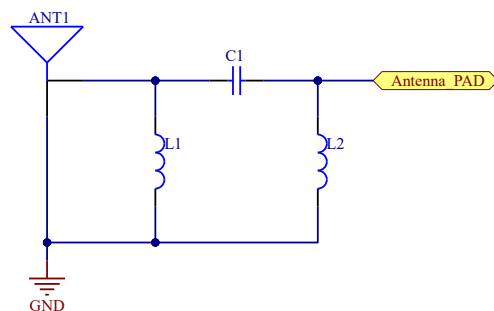
Figure 15: Minimal RF Matching Network Circuitry
