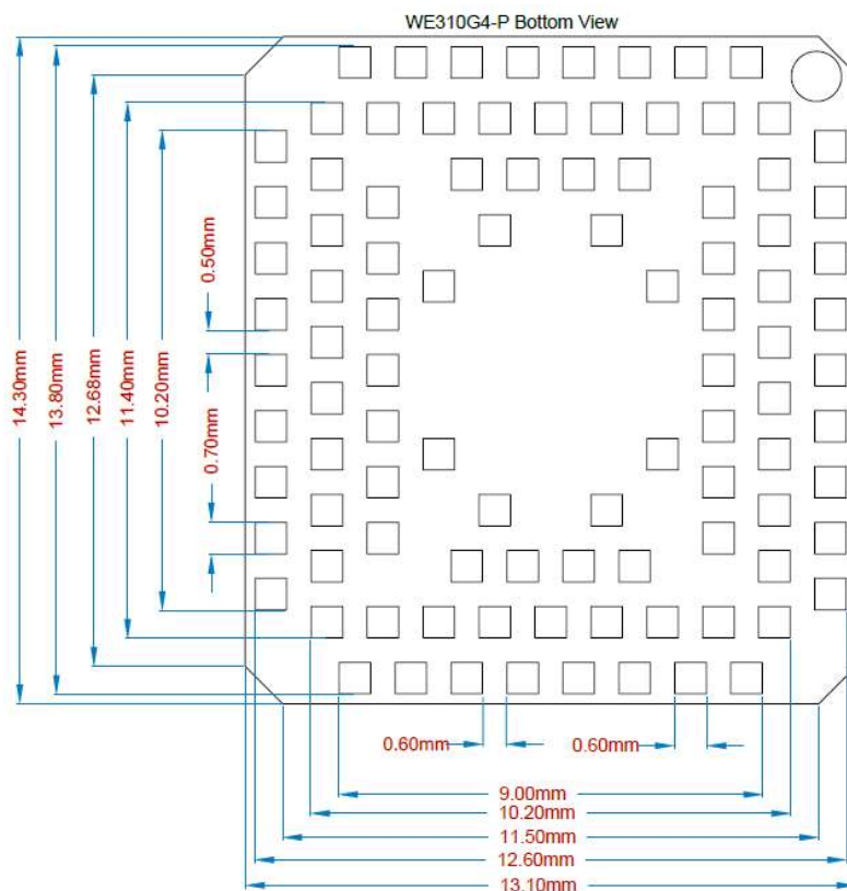
Figure 19: WE310G4-P Bottom View
