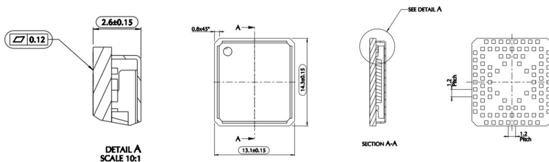
Figure 20: WE310G4-P Side View and Mechanical Design
