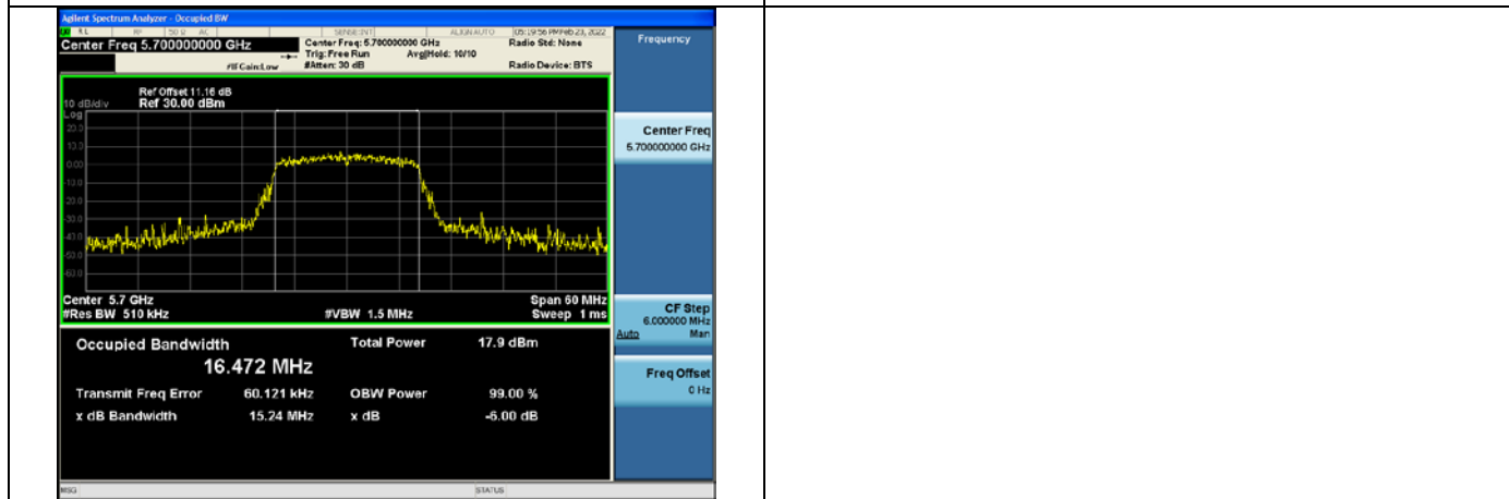
Test Mode:802.11a 5700MHz Chain0
