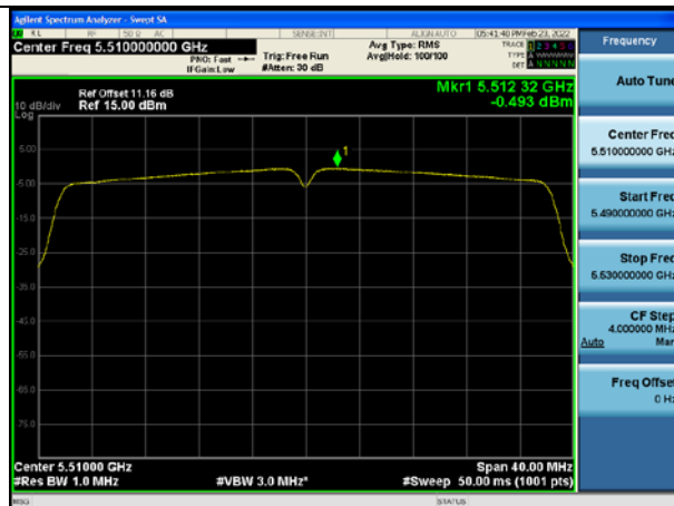
Test Mode:802.11ac VHT40 5510MHz Chain0
