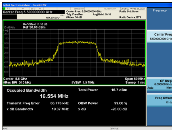
Test Mode:802.11a 5500MHz Chain0
