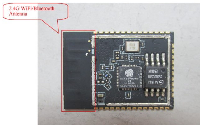
WiFi Modular Internal Photo
