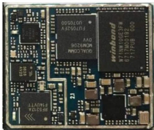
LTE Modular internal photo
