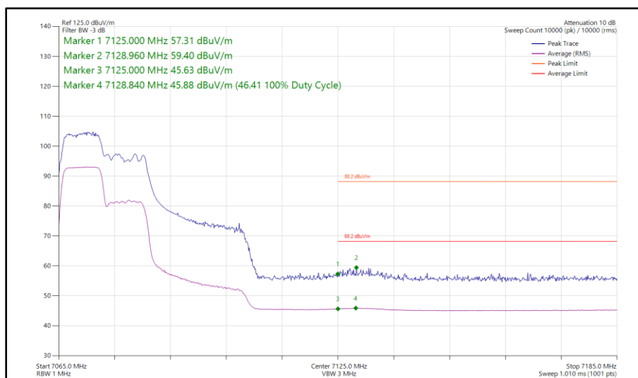
Figure 215 - 802.11ax HE40, RU 106-53, SISO, Core 0 - 7085 MHz Band Edge Frequency 7125 MHz
