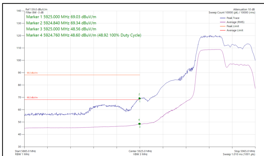
Figure 190 - 802.11ax HE20, RU 106-53, SISO, Core 0 - 5955 MHz Band Edge Frequency 5925 MHz
