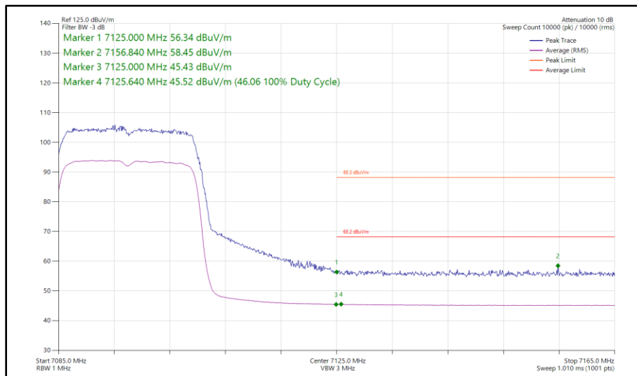
Figure 193 - 802.11ax HE20, SU, SISO, Core 0 - 7095 MHz Band Edge Frequency 7125 MHz
