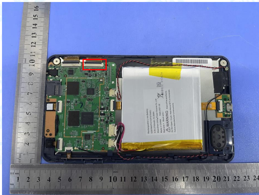
Photo 10 Internal of EUT-(7 inch)
