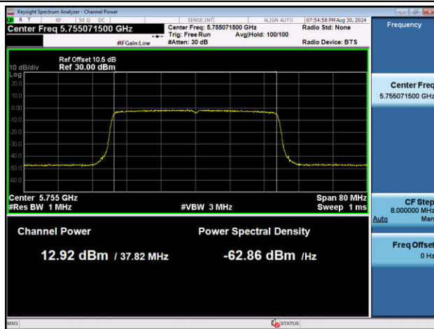
11AX40SISO-Ant2-5755-PASS
