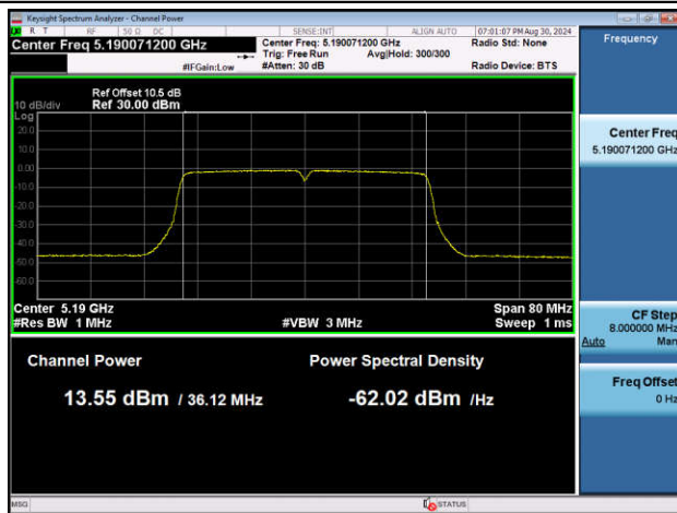
11AC40MIMO-Ant2-5190-PASS
