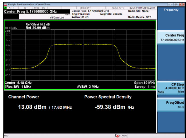
11AC20MIMO-Ant1-5180-PASS
