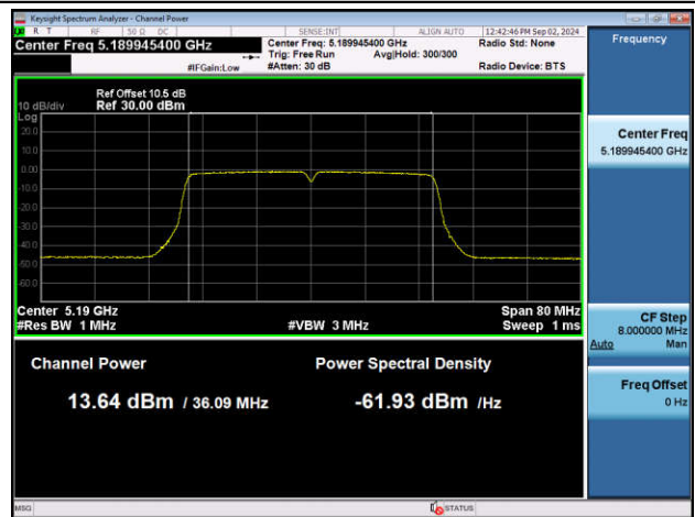
11AC40MIMO-Ant1-5190-PASS
