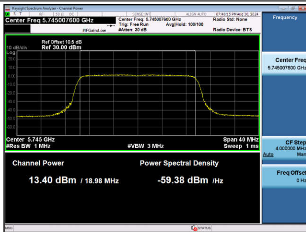
11AX20SISO-Ant2-5745-PASS
