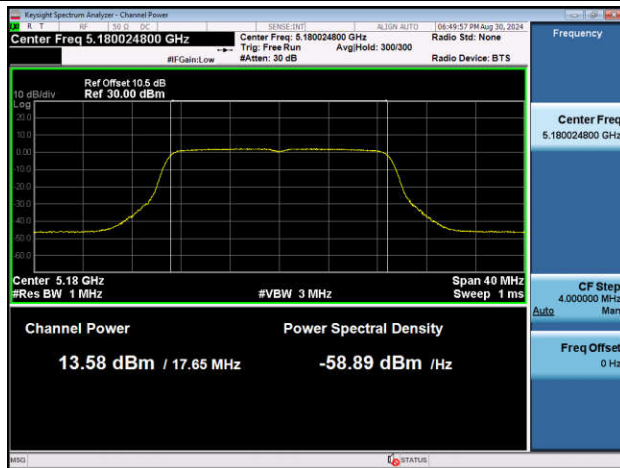
11AC20MIMO-Ant2-5180-PASS
