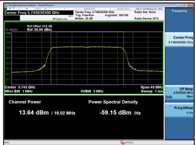
11AX20SISO-Ant1-5745-PASS
