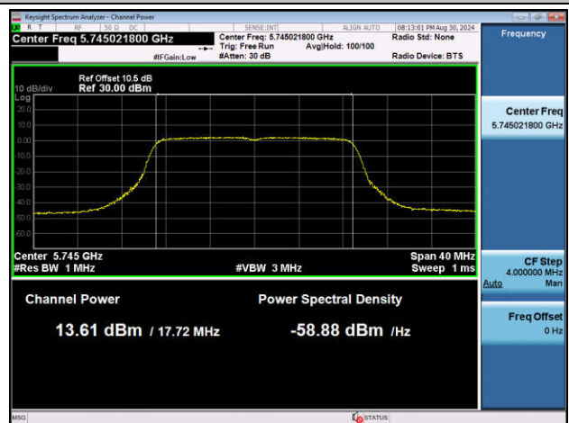
11AC20SISO-Ant1-5745-PASS
