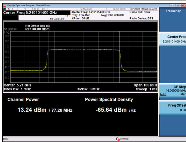
11AX80MIMO-Ant2-5210-PASS
