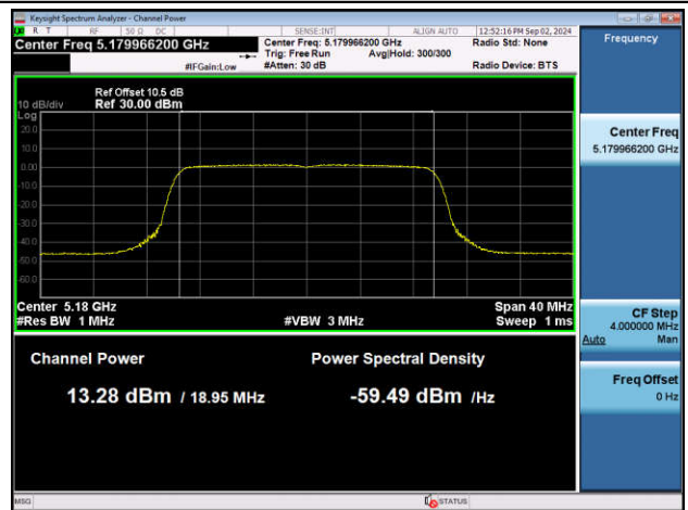
11AX20MIMO-Ant1-5180-PASS
