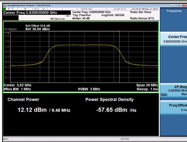
11A(10MHz)-Ant1-5820-PASS
