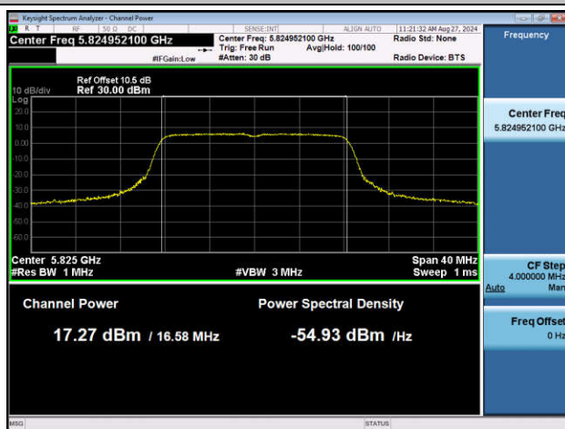
11A-Ant2-5825-PASS
