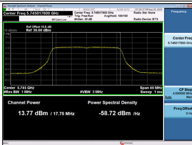
11AC20SISO-Ant2-5745-PASS
