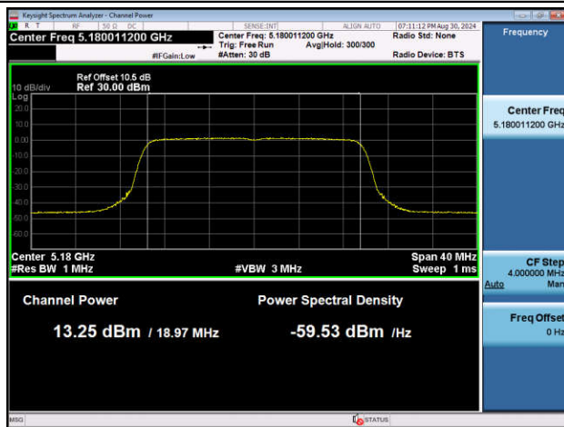
11AX20MIMO-Ant2-5180-PASS
