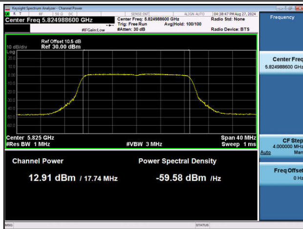
11N20SISO-Ant2-5825-PASS
