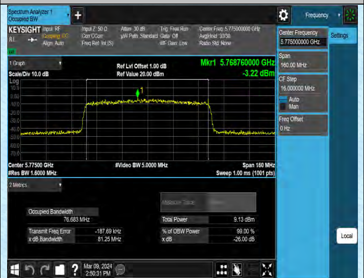
11AX80MIMO-Ant2-5775
