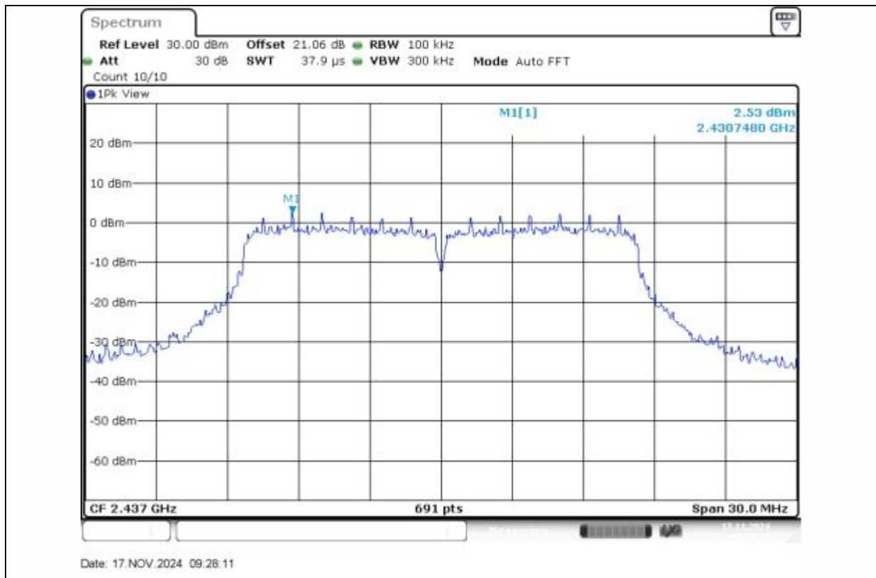
11G-Ant1-2437-0~Reference-PASS
