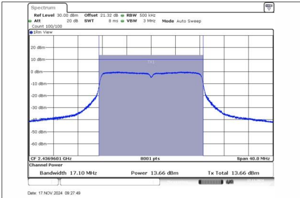
11G-Ant1-2437-PASS
