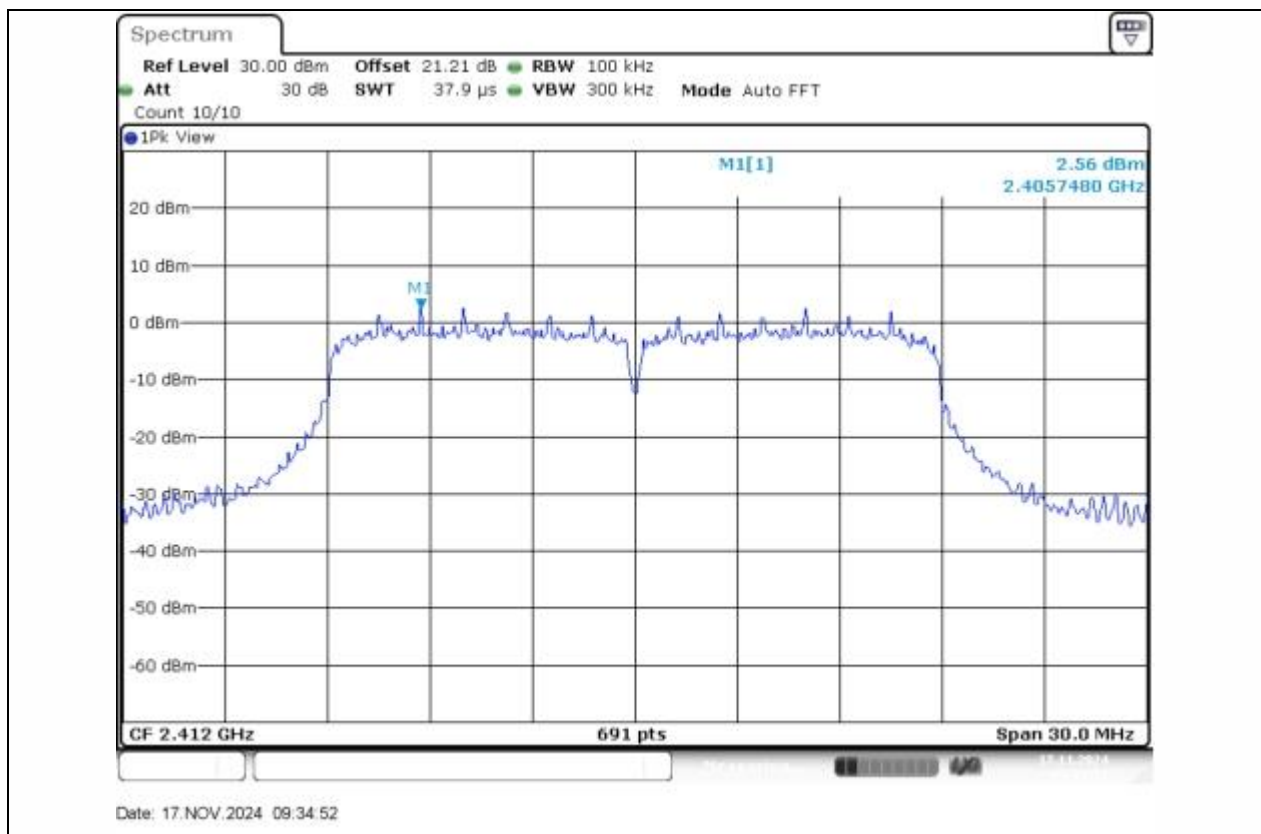
11N20SISO-Ant1-2412-0~Reference-PASS
