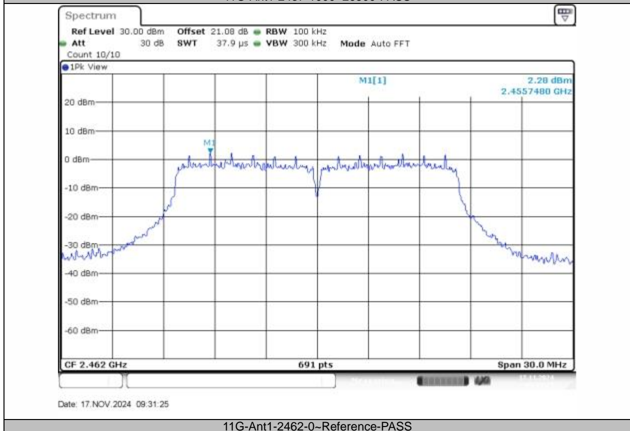
11G-Ant1-2462-0~Reference-PASS
