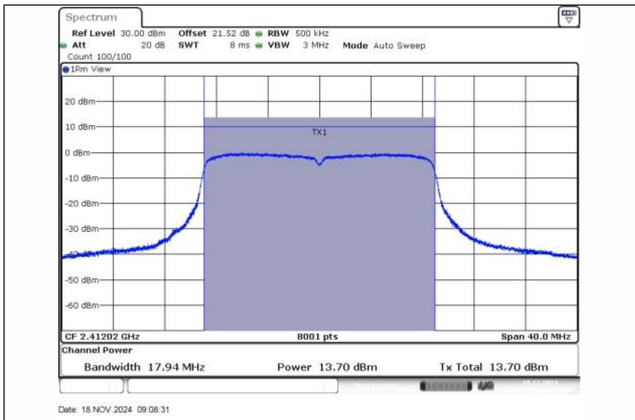
11N20SISO-Ant1-2412-PASS
