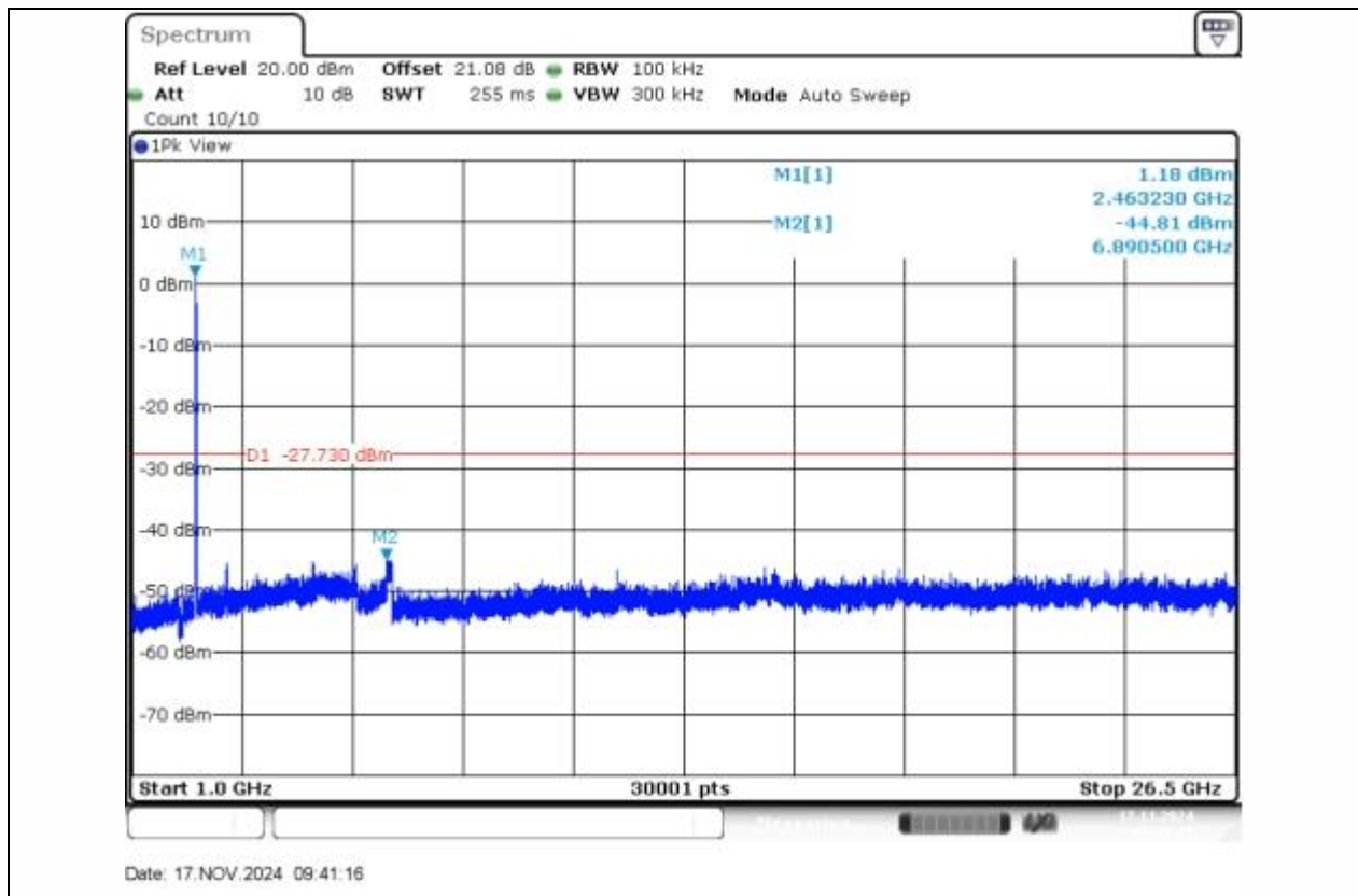
11N20SISO-Ant1-2462-1000~26500-PASS
