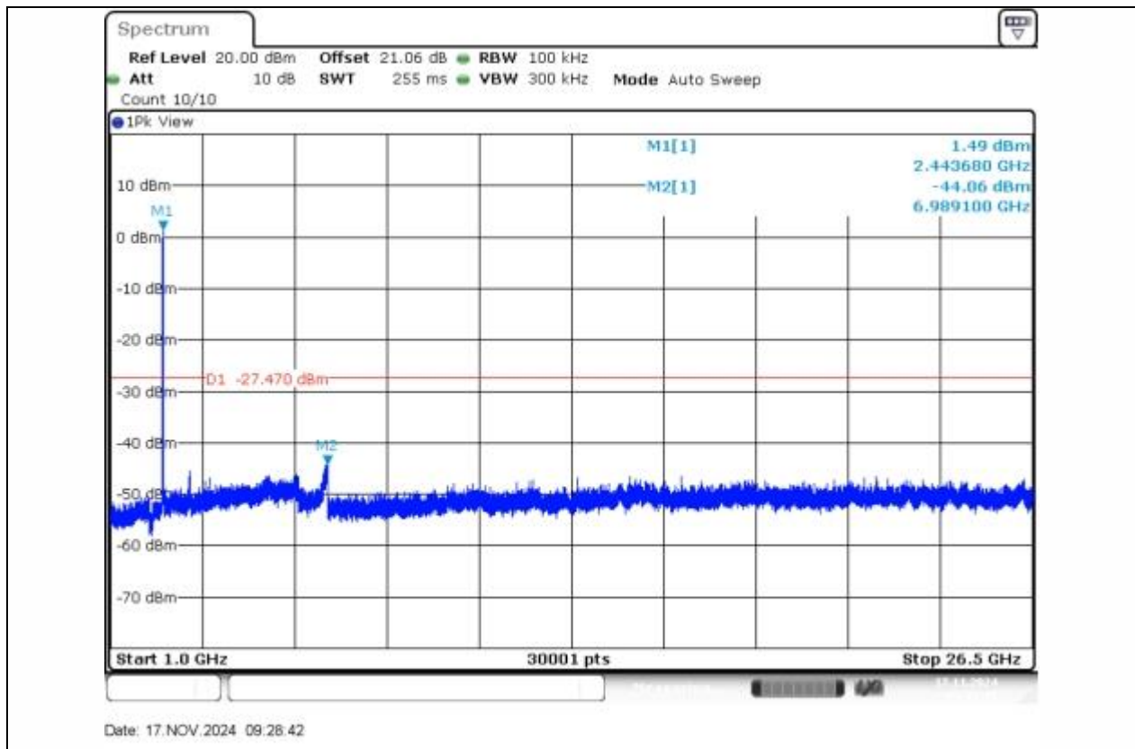
11G-Ant1-2437-1000~26500-PASS
