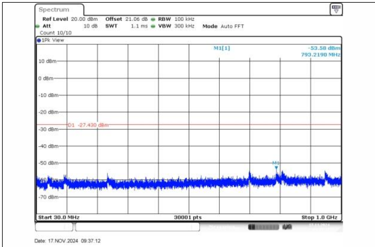
11N20SISO-Ant1-2437-30~1000-PASS
