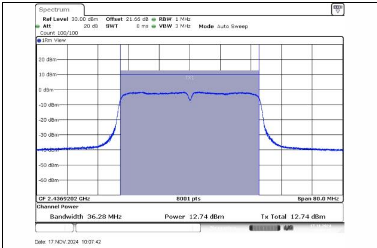
11N40SISO-Ant1-2437-PASS
