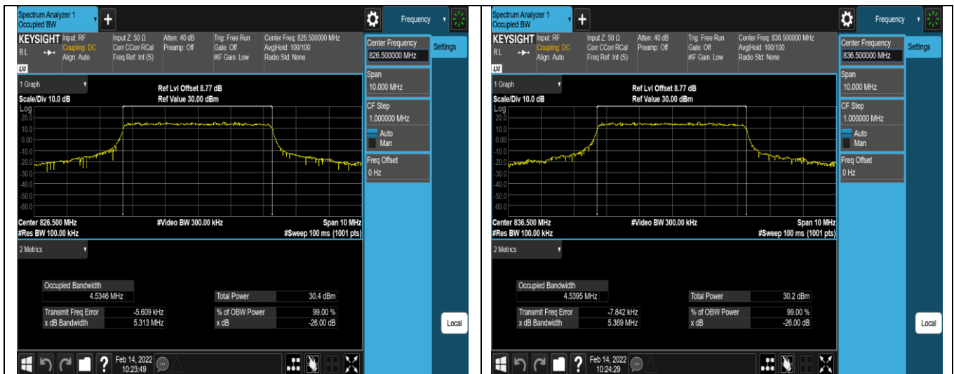
Band5-5MHz-QPSK-20625-25RB#0
