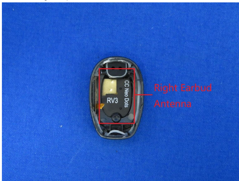
(21) EUT Photo-Right Earphone
